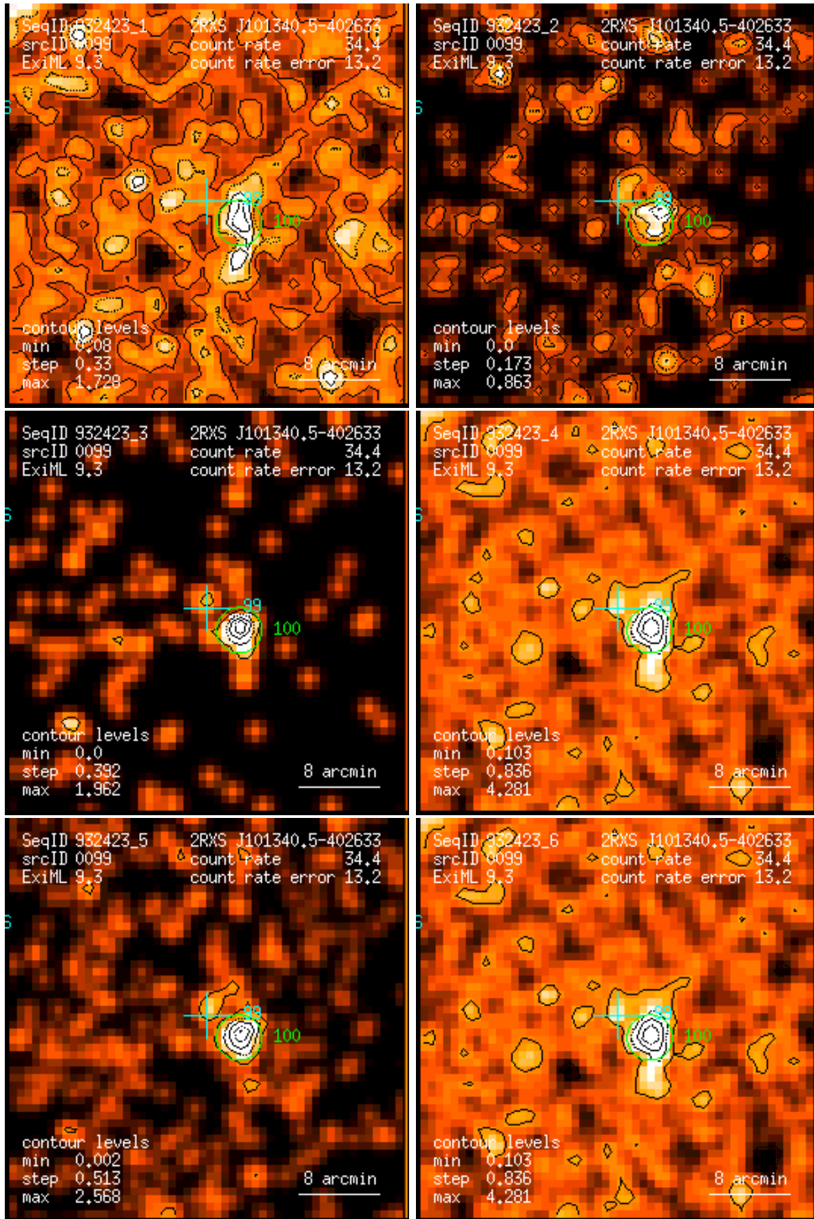
Figure 99: RASS 932423: detection 0099: band rate images, Gaussian filter: (1) PSPC channels 11 – 41, (2) 52 – 90, (3) 91 – 201, (4) 11 – 235, (5) 52 – 201, (6) 11 – 201. Broad band rates in counts/ks. Band rate contour levels in counts/ks/arcmin 2 .
