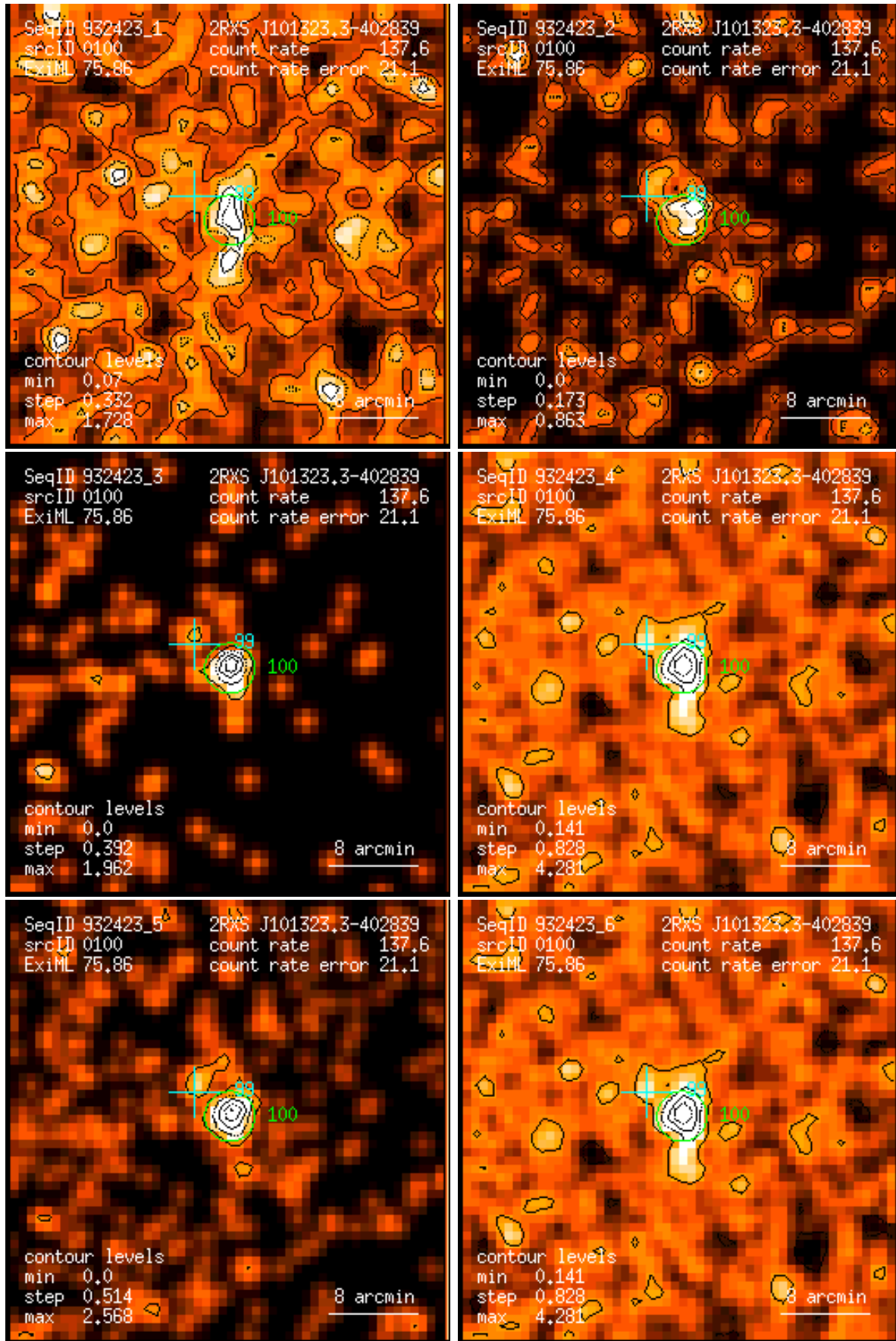
Figure 100: RASS 932423: detection 0100: band rate images, Gaussian filter: (1) PSPC channels 11 – 41, (2) 52 – 90, (3) 91 – 201, (4) 11 – 235, (5) 52 – 201, (6) 11 – 201. Broad band rates in counts/ks. Band rate contour levels in counts/ks/arcmin 2 .
