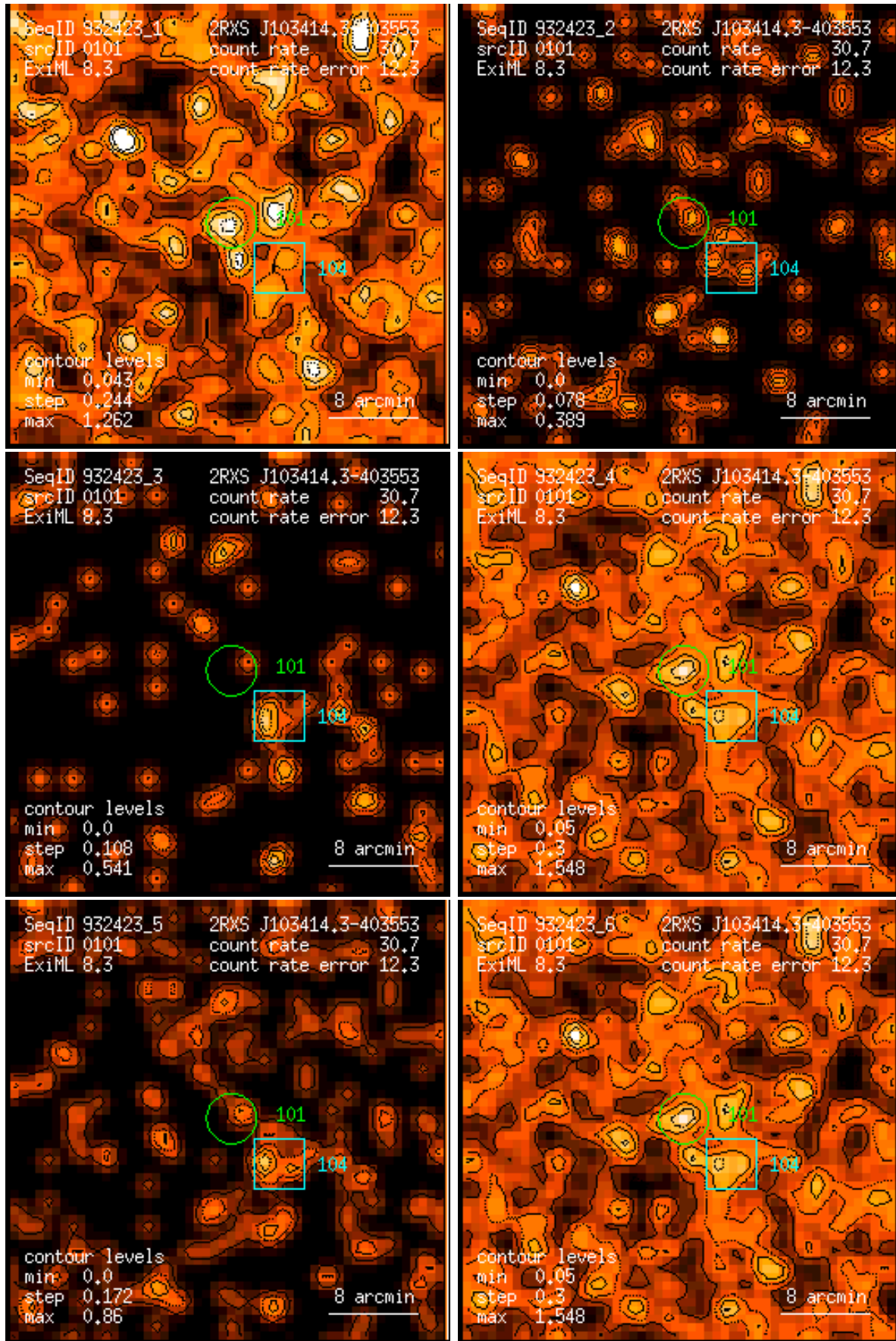
Figure 101: RASS 932423: detection 0101: band rate images, Gaussian filter: (1) PSPC channels 11 – 41, (2) 52 – 90, (3) 91 – 201, (4) 11 – 235, (5) 52 – 201, (6) 11 – 201. Broad band rates in counts/ks. Band rate contour levels in counts/ks/arcmin 2 .
