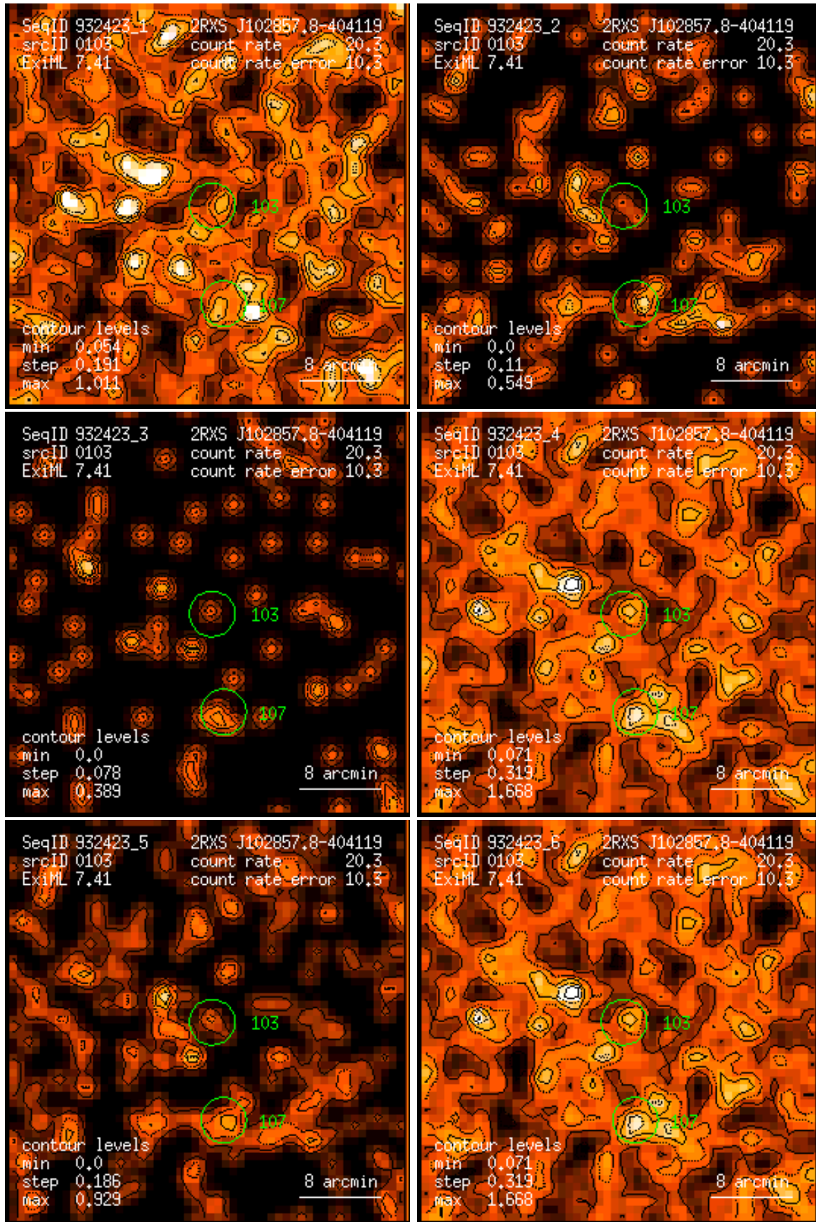
Figure 103: RASS 932423: detection 0103: band rate images, Gaussian filter: (1) PSPC channels 11 – 41, (2) 52 – 90, (3) 91 – 201, (4) 11 – 235, (5) 52 – 201, (6) 11 – 201. Broad band rates in counts/ks. Band rate contour levels in counts/ks/arcmin 2 .
