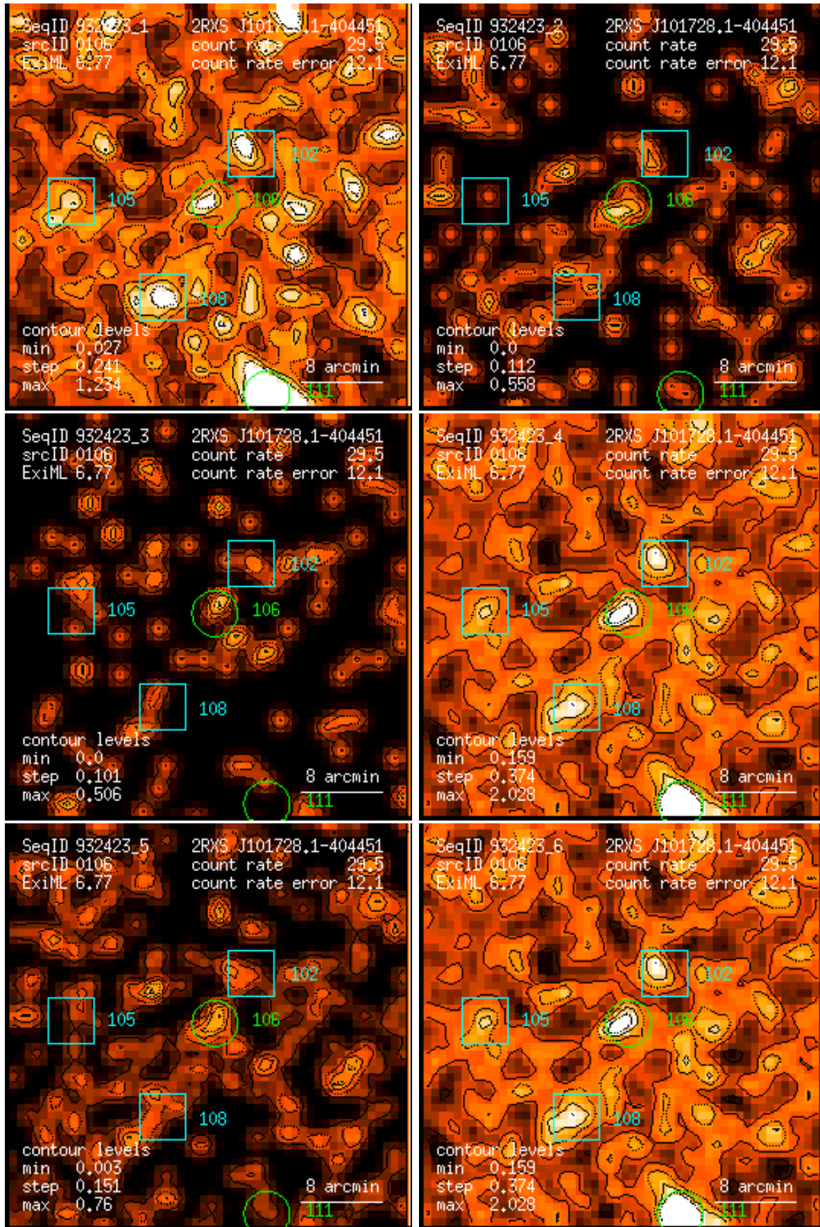
Figure 106: RASS 932423: detection 0106: band rate images, Gaussian filter: (1) PSPC channels 11 – 41, (2) 52 – 90, (3) 91 – 201, (4) 11 – 235, (5) 52 – 201, (6) 11 – 201. Broad band rates in counts/ks. Band rate contour levels in counts/ks/arcmin 2 .
