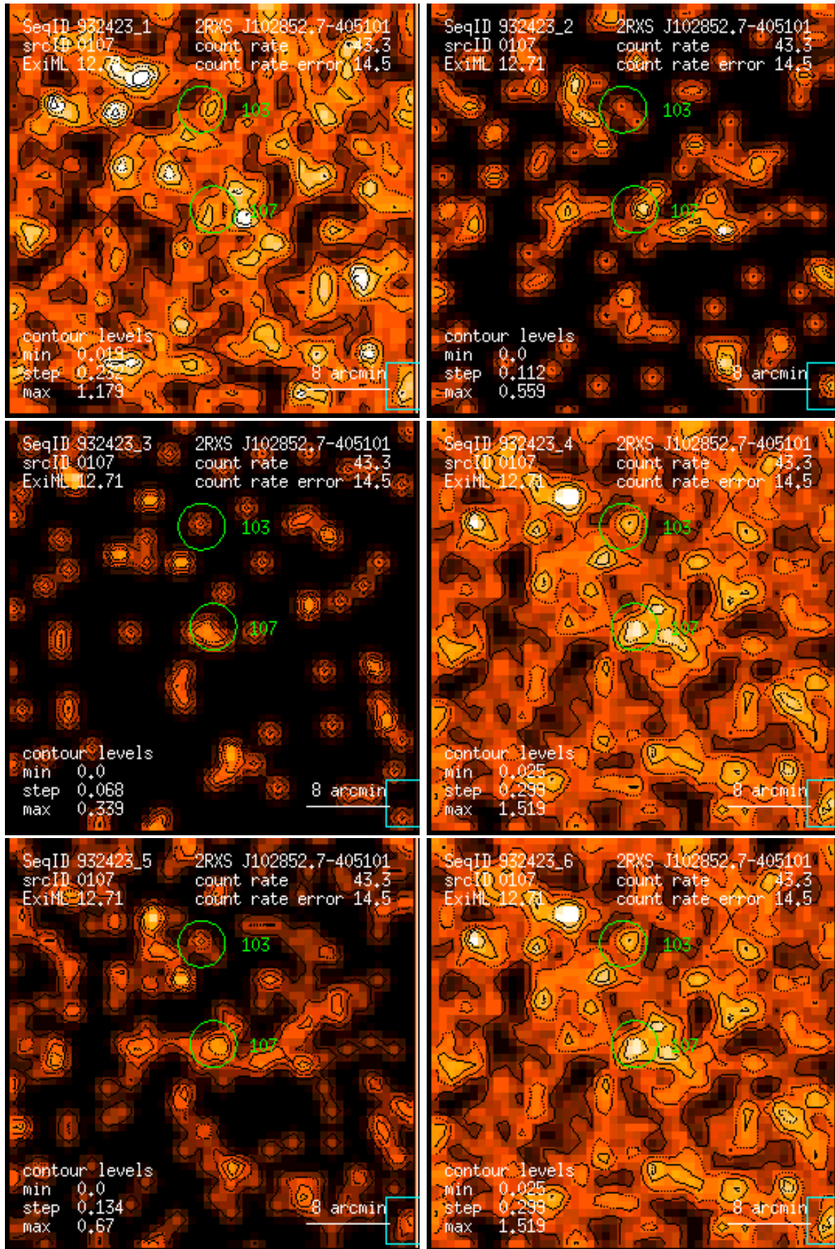
Figure 107: RASS 932423: detection 0107: band rate images, Gaussian filter: (1) PSPC channels 11 – 41, (2) 52 – 90, (3) 91 – 201, (4) 11 – 235, (5) 52 – 201, (6) 11 – 201. Broad band rates in counts/ks. Band rate contour levels in counts/ks/arcmin 2 .
