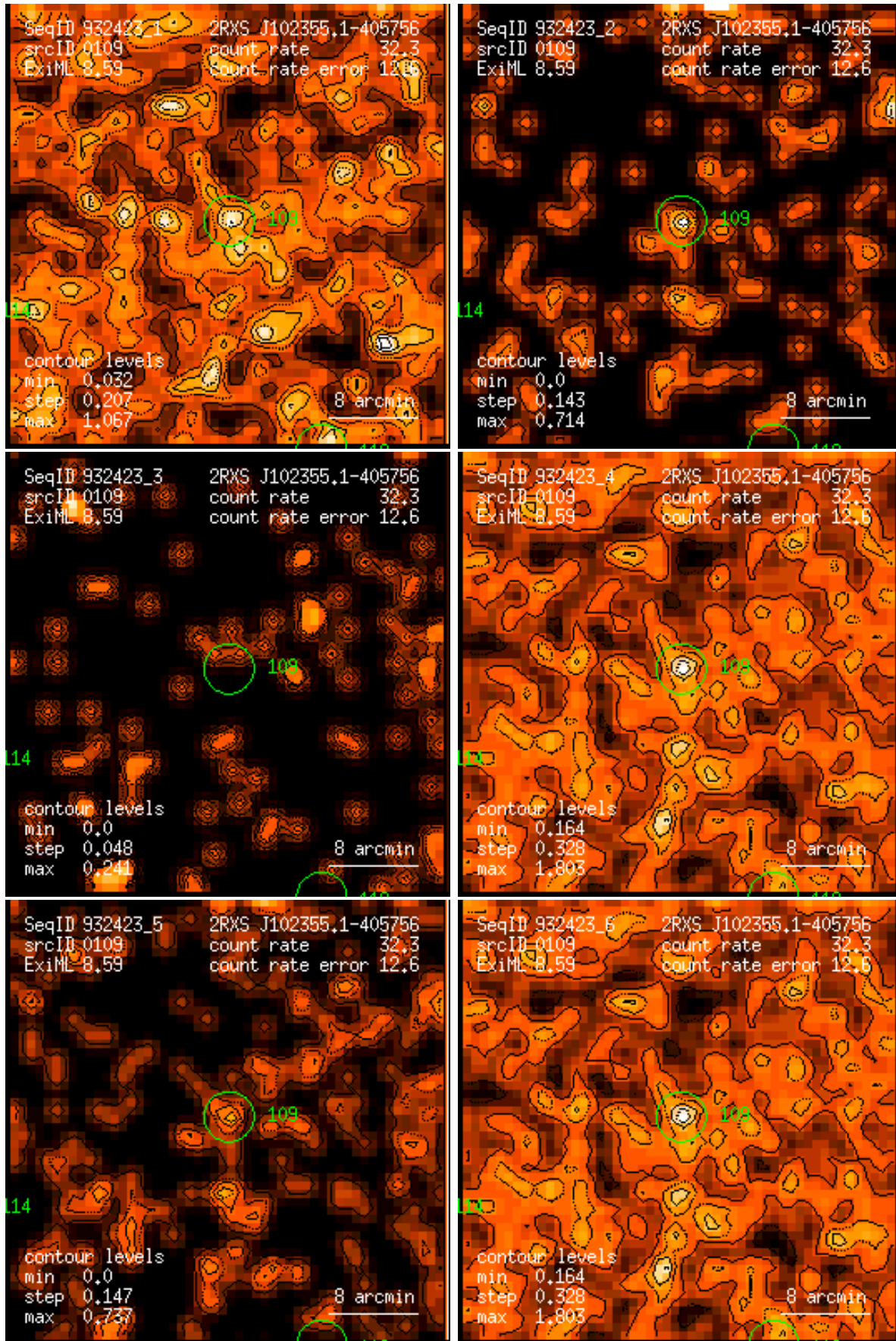
Figure 109: RASS 932423: detection 0109: band rate images, Gaussian filter: (1) PSPC channels 11 – 41, (2) 52 – 90, (3) 91 – 201, (4) 11 – 235, (5) 52 – 201, (6) 11 – 201. Broad band rates in counts/ks. Band rate contour levels in counts/ks/arcmin 2 .
