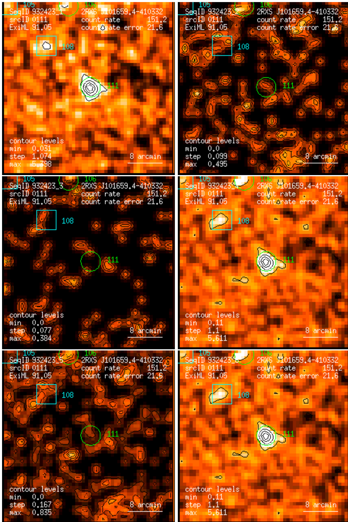
Figure 111: RASS 932423: detection 0111: band rate images, Gaussian filter: (1) PSPC channels 11 – 41, (2) 52 – 90, (3) 91 – 201, (4) 11 – 235, (5) 52 – 201, (6) 11 – 201. Broad band rates in counts/ks. Band rate contour levels in counts/ks/arcmin 2 .
