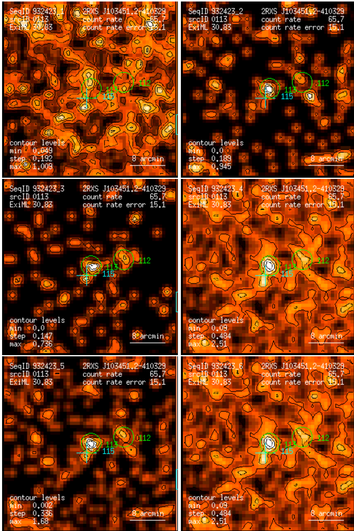
Figure 113: RASS 932423: detection 0113: band rate images, Gaussian filter: (1) PSPC channels 11 – 41, (2) 52 – 90, (3) 91 – 201, (4) 11 – 235, (5) 52 – 201, (6) 11 – 201. Broad band rates in counts/ks. Band rate contour levels in counts/ks/arcmin 2 .
