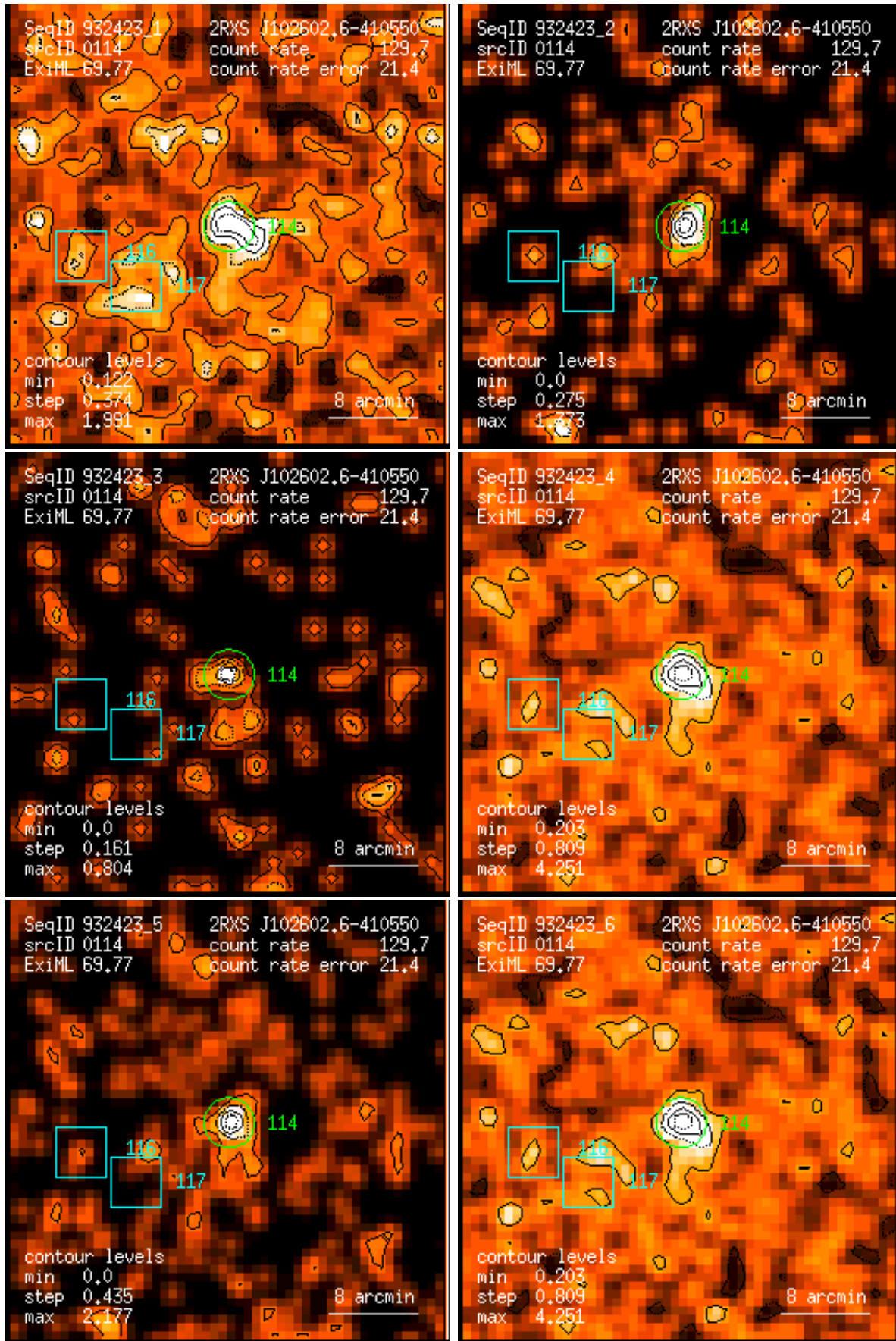
Figure 114: RASS 932423: detection 0114: band rate images, Gaussian filter: (1) PSPC channels 11 – 41, (2) 52 – 90, (3) 91 – 201, (4) 11 – 235, (5) 52 – 201, (6) 11 – 201. Broad band rates in counts/ks. Band rate contour levels in counts/ks/arcmin 2 .
