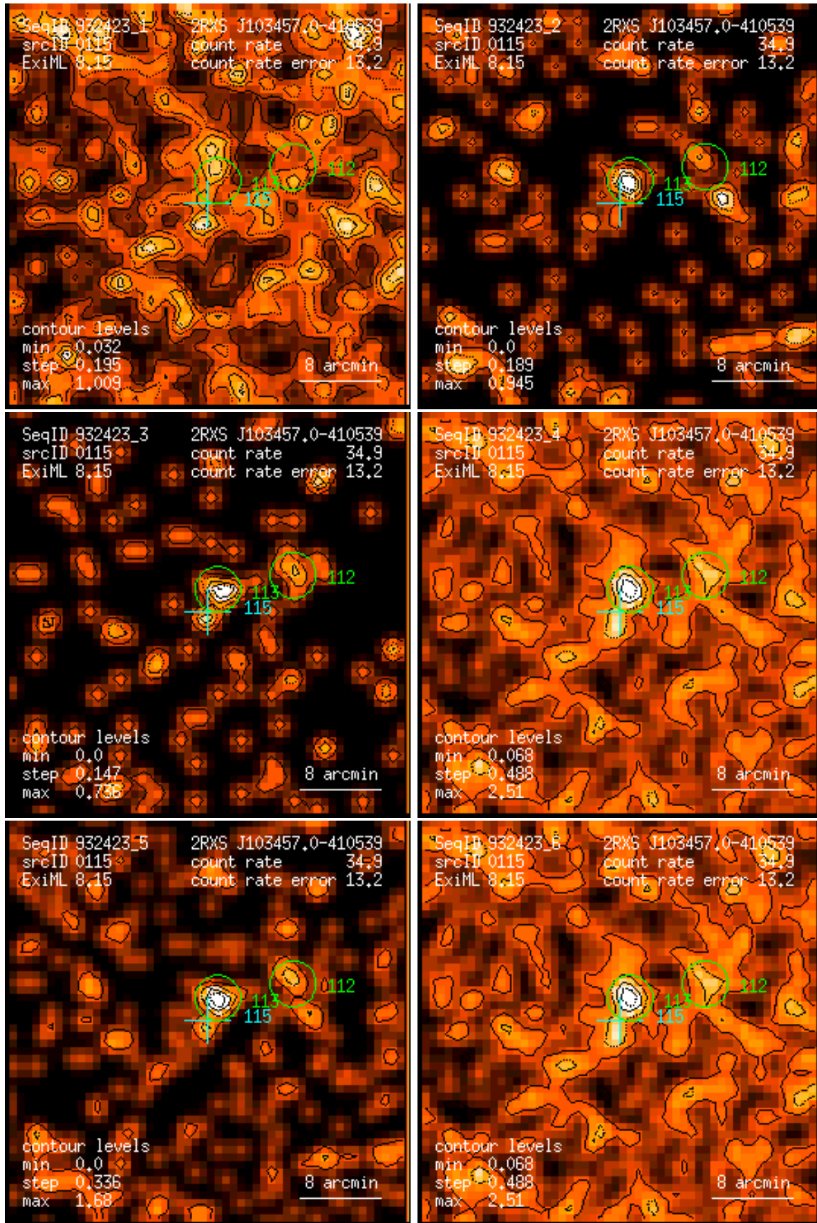
Figure 115: RASS 932423: detection 0115: band rate images, Gaussian filter: (1) PSPC channels 11 – 41, (2) 52 – 90, (3) 91 – 201, (4) 11 – 235, (5) 52 – 201, (6) 11 – 201. Broad band rates in counts/ks. Band rate contour levels in counts/ks/arcmin 2 .
