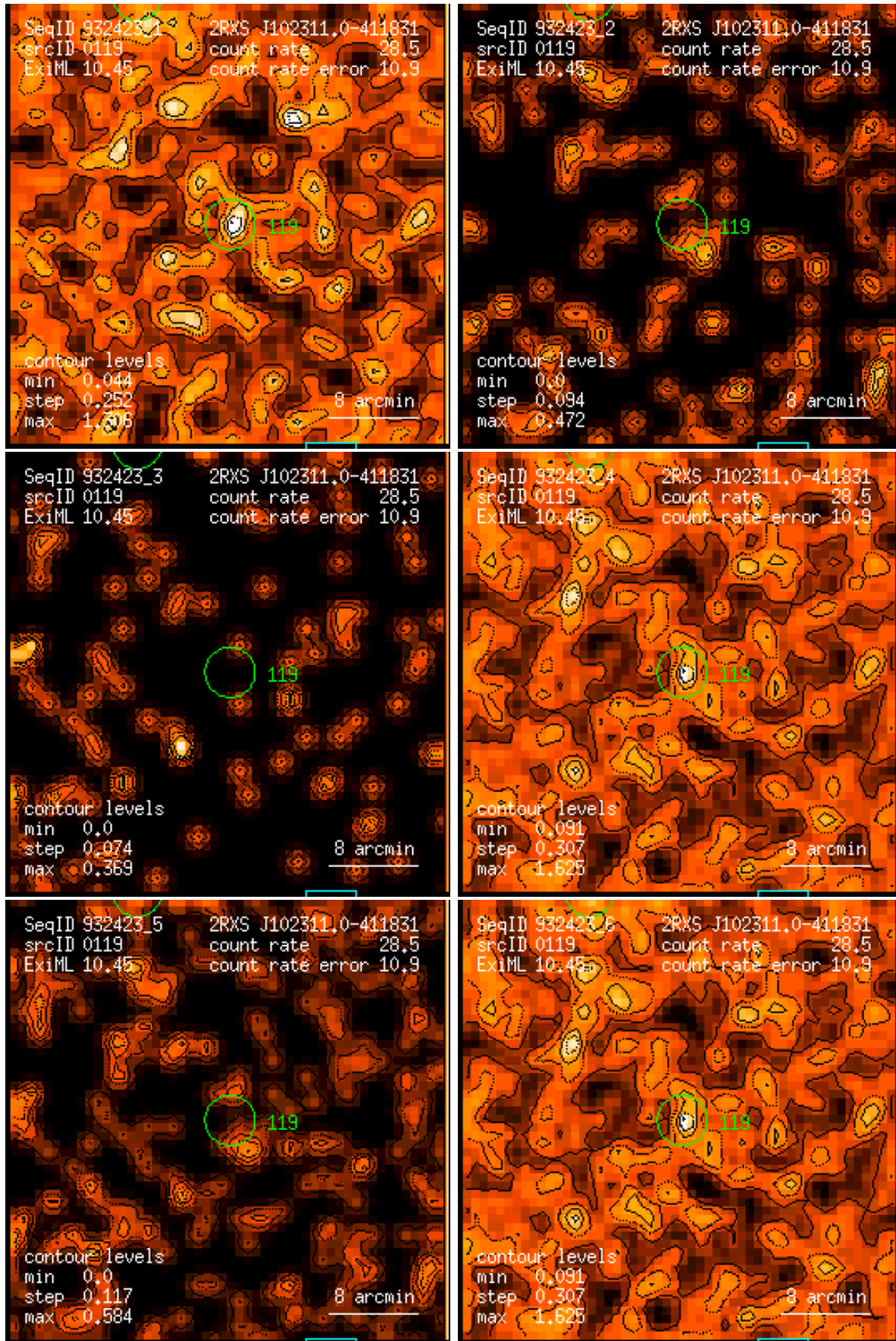
Figure 119: RASS 932423: detection 0119: band rate images, Gaussian filter: (1) PSPC channels 11 – 41, (2) 52 – 90, (3) 91 – 201, (4) 11 – 235, (5) 52 – 201, (6) 11 – 201. Broad band rates in counts/ks. Band rate contour levels in counts/ks/arcmin 2 .
