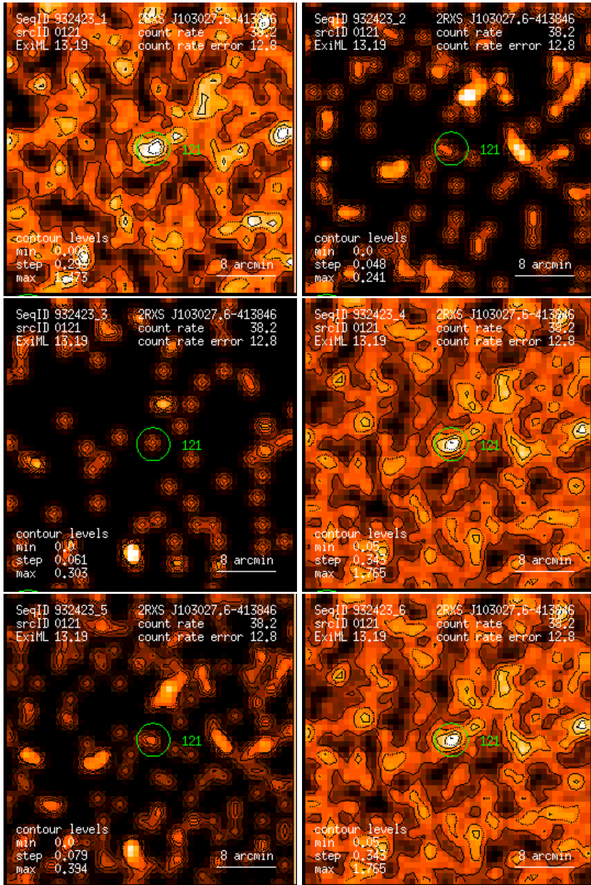
Figure 121: RASS 932423: detection 0121: band rate images, Gaussian filter: (1) PSPC channels 11 – 41, (2) 52 – 90, (3) 91 – 201, (4) 11 – 235, (5) 52 – 201, (6) 11 – 201. Broad band rates in counts/ks. Band rate contour levels in counts/ks/arcmin 2 .
