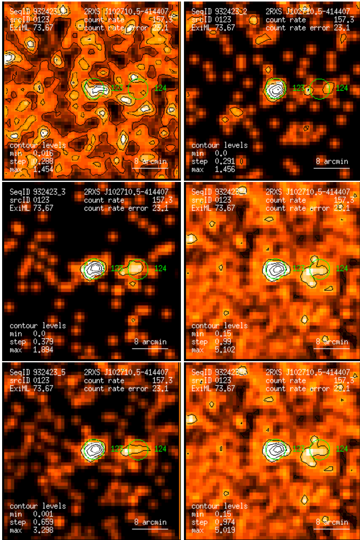
Figure 123: RASS 932423: detection 0123: band rate images, Gaussian filter: (1) PSPC channels 11 – 41, (2) 52 – 90, (3) 91 – 201, (4) 11 – 235, (5) 52 – 201, (6) 11 – 201. Broad band rates in counts/ks. Band rate contour levels in counts/ks/arcmin 2 .
