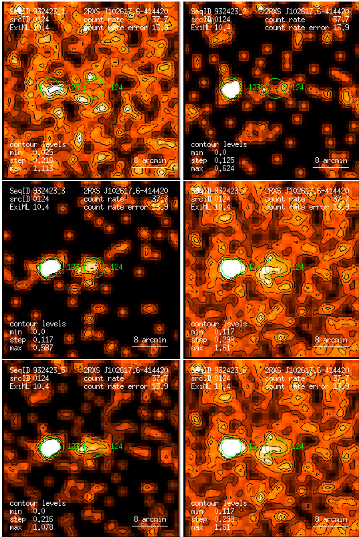
Figure 124: RASS 932423: detection 0124: band rate images, Gaussian filter: (1) PSPC channels 11 – 41, (2) 52 – 90, (3) 91 – 201, (4) 11 – 235, (5) 52 – 201, (6) 11 – 201. Broad band rates in counts/ks. Band rate contour levels in counts/ks/arcmin 2 .
