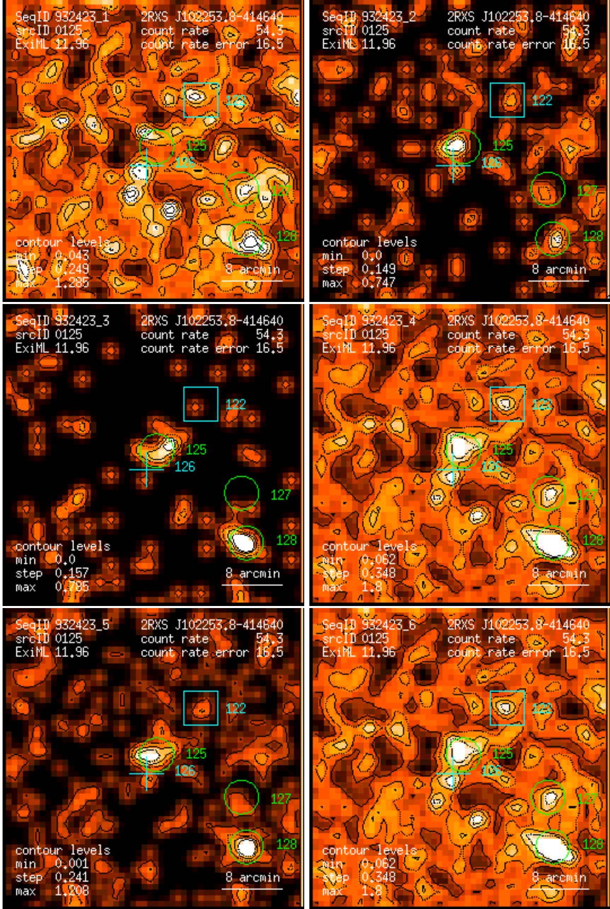
Figure 125: RASS 932423: detection 0125: band rate images, Gaussian filter: (1) PSPC channels 11 – 41, (2) 52 – 90, (3) 91 – 201, (4) 11 – 235, (5) 52 – 201, (6) 11 – 201. Broad band rates in counts/ks. Band rate contour levels in counts/ks/arcmin 2 .
