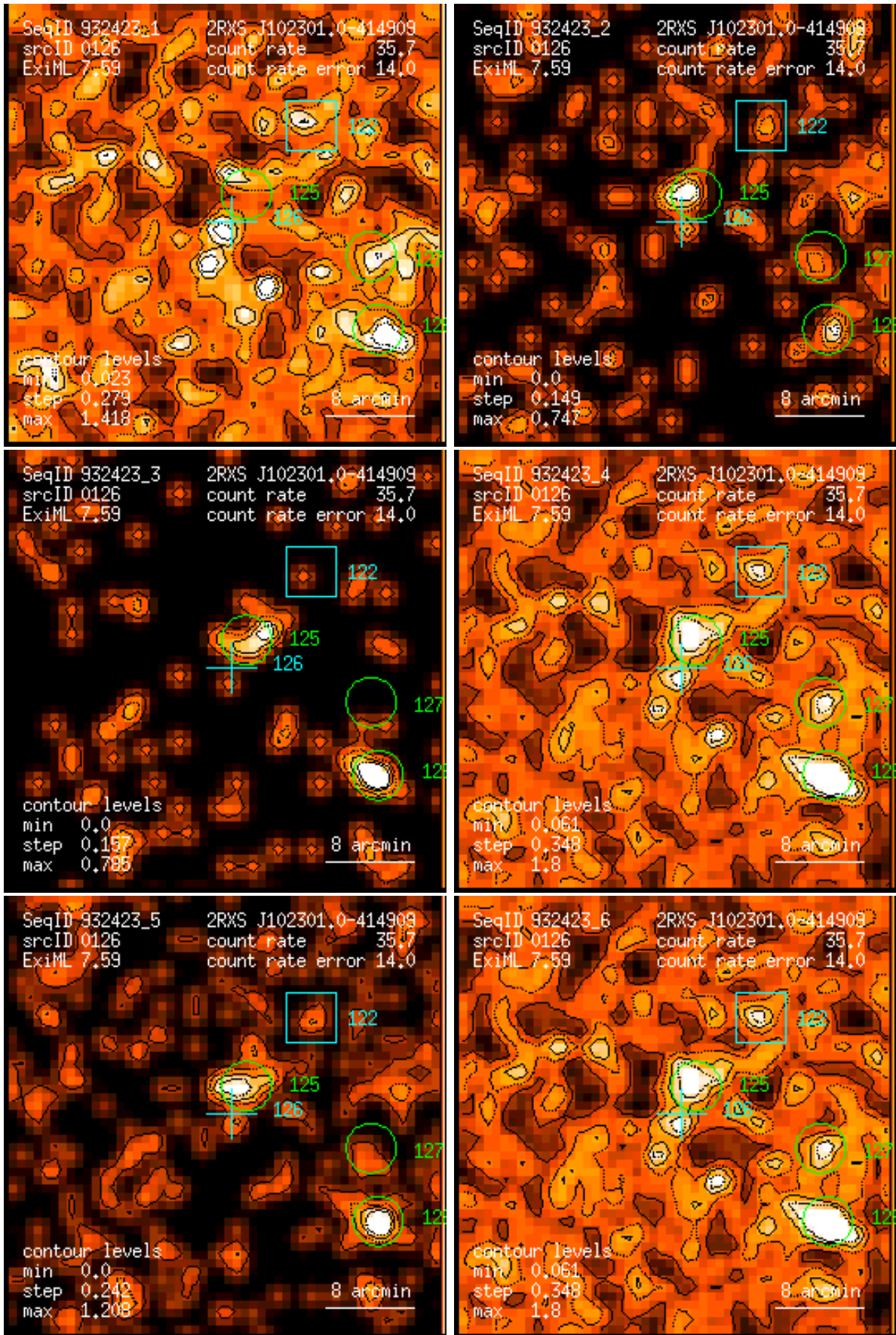
Figure 126: RASS 932423: detection 0126: band rate images, Gaussian filter: (1) PSPC channels 11 – 41, (2) 52 – 90, (3) 91 – 201, (4) 11 – 235, (5) 52 – 201, (6) 11 – 201. Broad band rates in counts/ks. Band rate contour levels in counts/ks/arcmin 2 .
