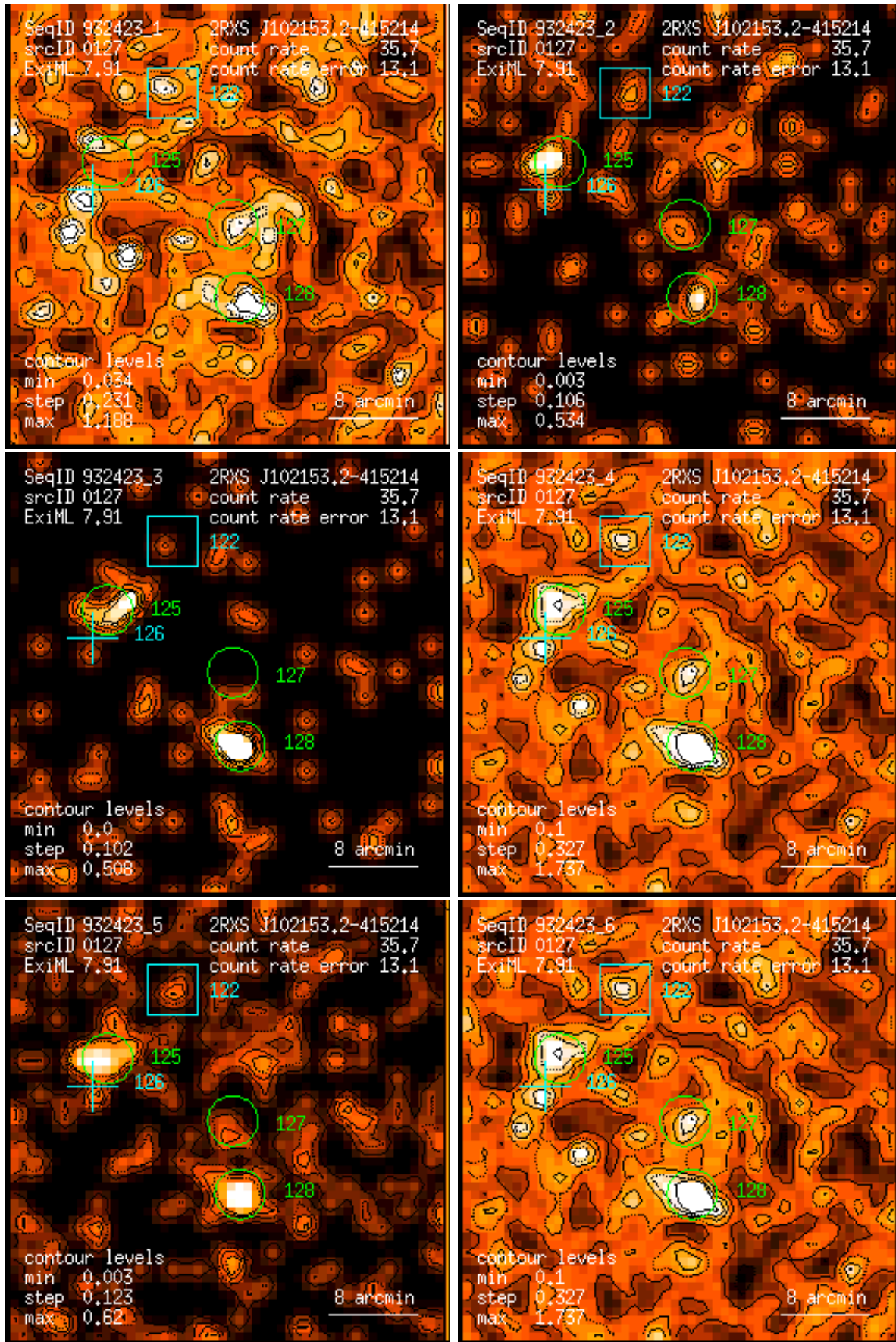
Figure 127: RASS 932423: detection 0127: band rate images, Gaussian filter: (1) PSPC channels 11 – 41, (2) 52 – 90, (3) 91 – 201, (4) 11 – 235, (5) 52 – 201, (6) 11 – 201. Broad band rates in counts/ks. Band rate contour levels in counts/ks/arcmin 2 .
