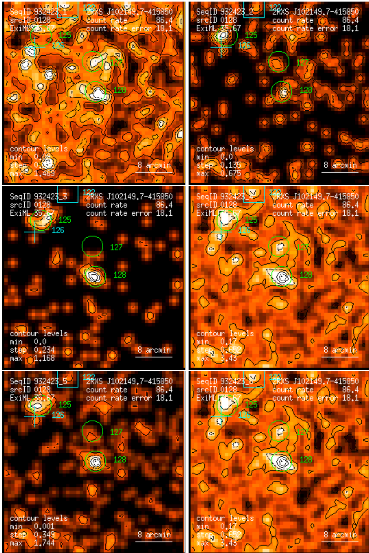
Figure 128: RASS 932423: detection 0128: band rate images, Gaussian filter: (1) PSPC channels 11 – 41, (2) 52 – 90, (3) 91 – 201, (4) 11 – 235, (5) 52 – 201, (6) 11 – 201. Broad band rates in counts/ks. Band rate contour levels in counts/ks/arcmin 2 .
