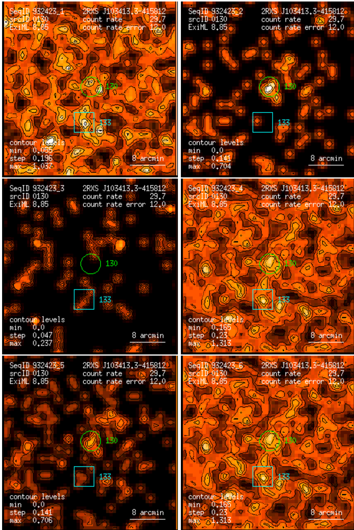
Figure 130: RASS 932423: detection 0130: band rate images, Gaussian filter: (1) PSPC channels 11 – 41, (2) 52 – 90, (3) 91 – 201, (4) 11 – 235, (5) 52 – 201, (6) 11 – 201. Broad band rates in counts/ks. Band rate contour levels in counts/ks/arcmin 2 .
