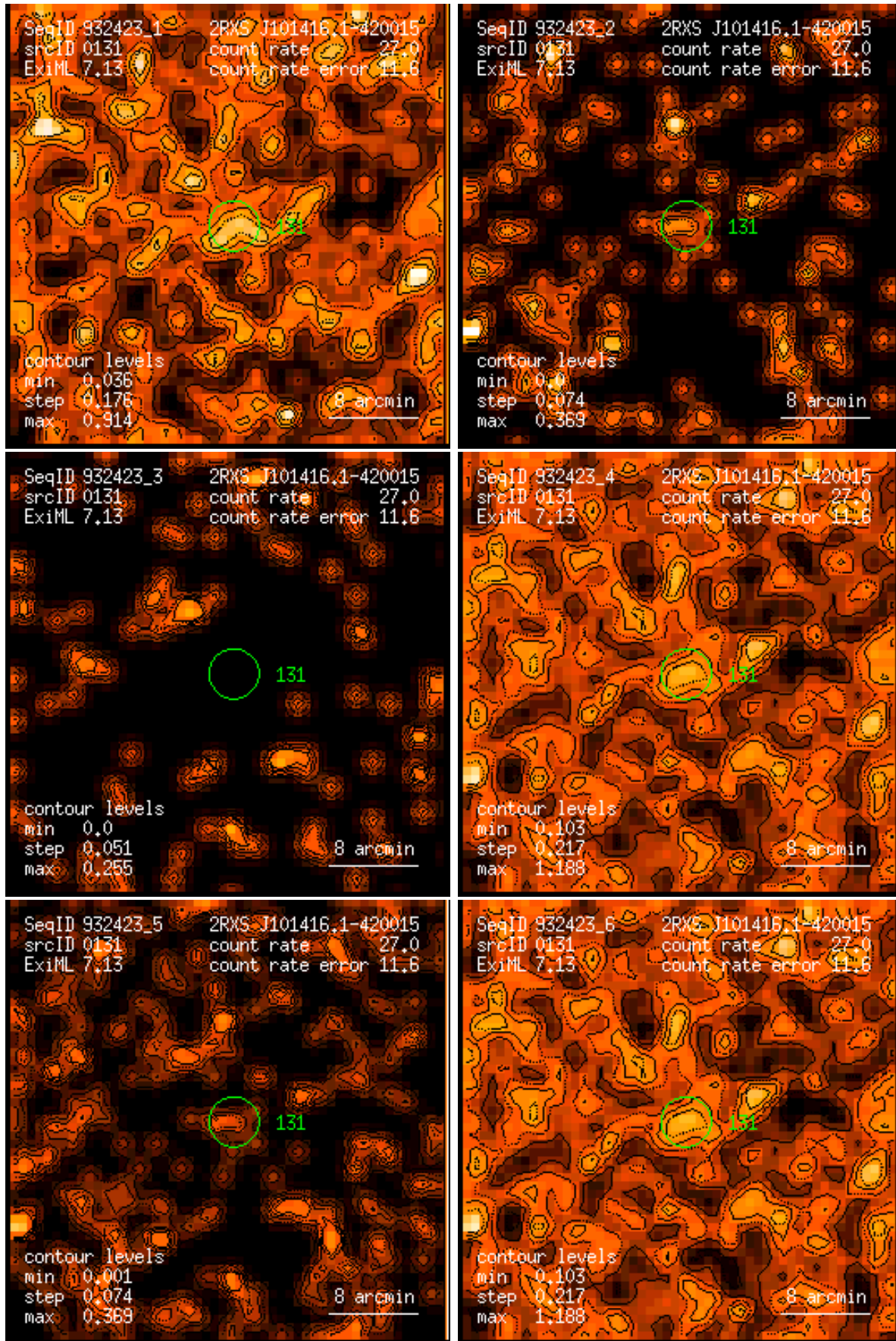
Figure 131: RASS 932423: detection 0131: band rate images, Gaussian filter: (1) PSPC channels 11 – 41, (2) 52 – 90, (3) 91 – 201, (4) 11 – 235, (5) 52 – 201, (6) 11 – 201. Broad band rates in counts/ks. Band rate contour levels in counts/ks/arcmin 2 .
