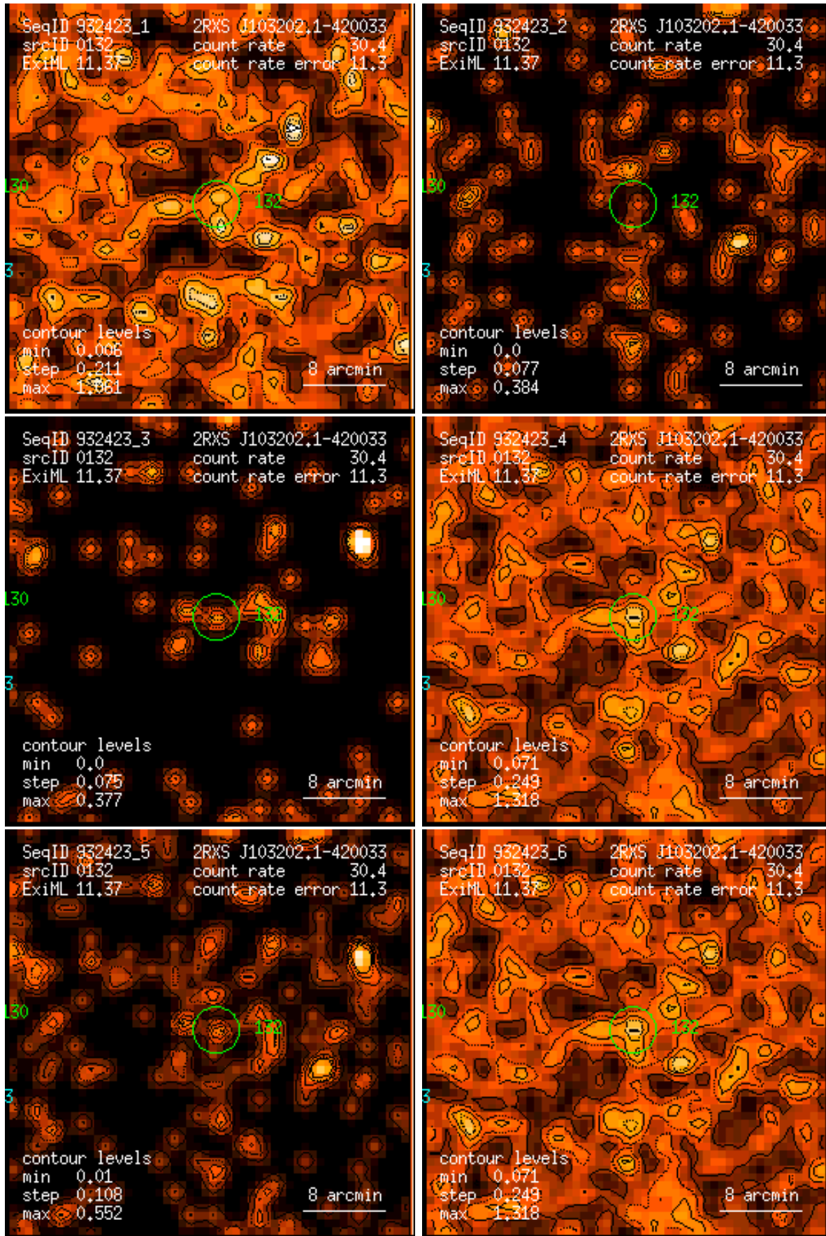
Figure 132: RASS 932423: detection 0132: band rate images, Gaussian filter: (1) PSPC channels 11 – 41, (2) 52 – 90, (3) 91 – 201, (4) 11 – 235, (5) 52 – 201, (6) 11 – 201. Broad band rates in counts/ks. Band rate contour levels in counts/ks/arcmin 2 .
