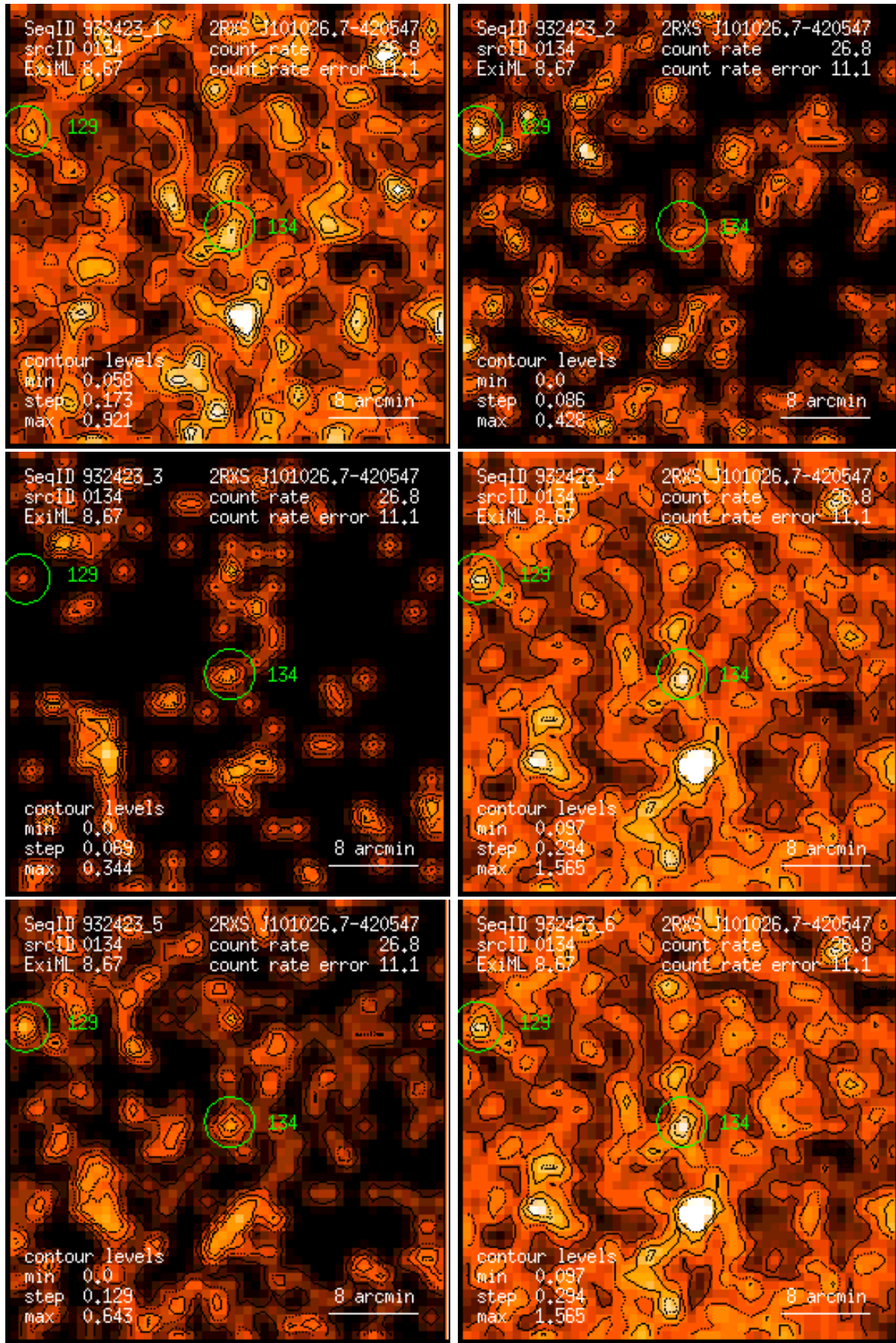
Figure 134: RASS 932423: detection 0134: band rate images, Gaussian filter: (1) PSPC channels 11 – 41, (2) 52 – 90, (3) 91 – 201, (4) 11 – 235, (5) 52 – 201, (6) 11 – 201. Broad band rates in counts/ks. Band rate contour levels in counts/ks/arcmin 2 .
