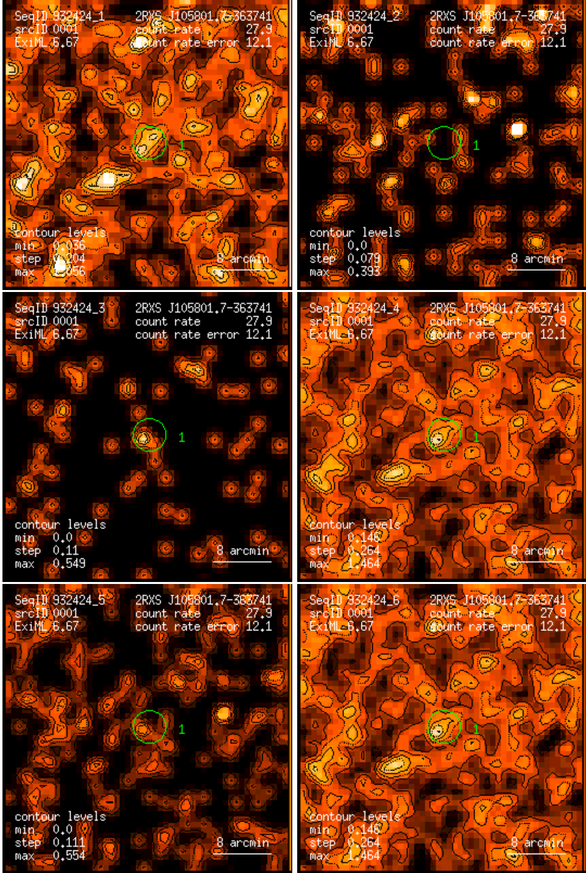
Figure 1: RASS 932424: detection 0001: band rate images, Gaussian filter: (1) PSPC channels 11 – 41, (2) 52 – 90, (3) 91 – 201, (4) 11 – 235, (5) 52 – 201, (6) 11 – 201. Broad band rates in counts/ks. Band rate contour levels in counts/ks/arcmin 2 .
