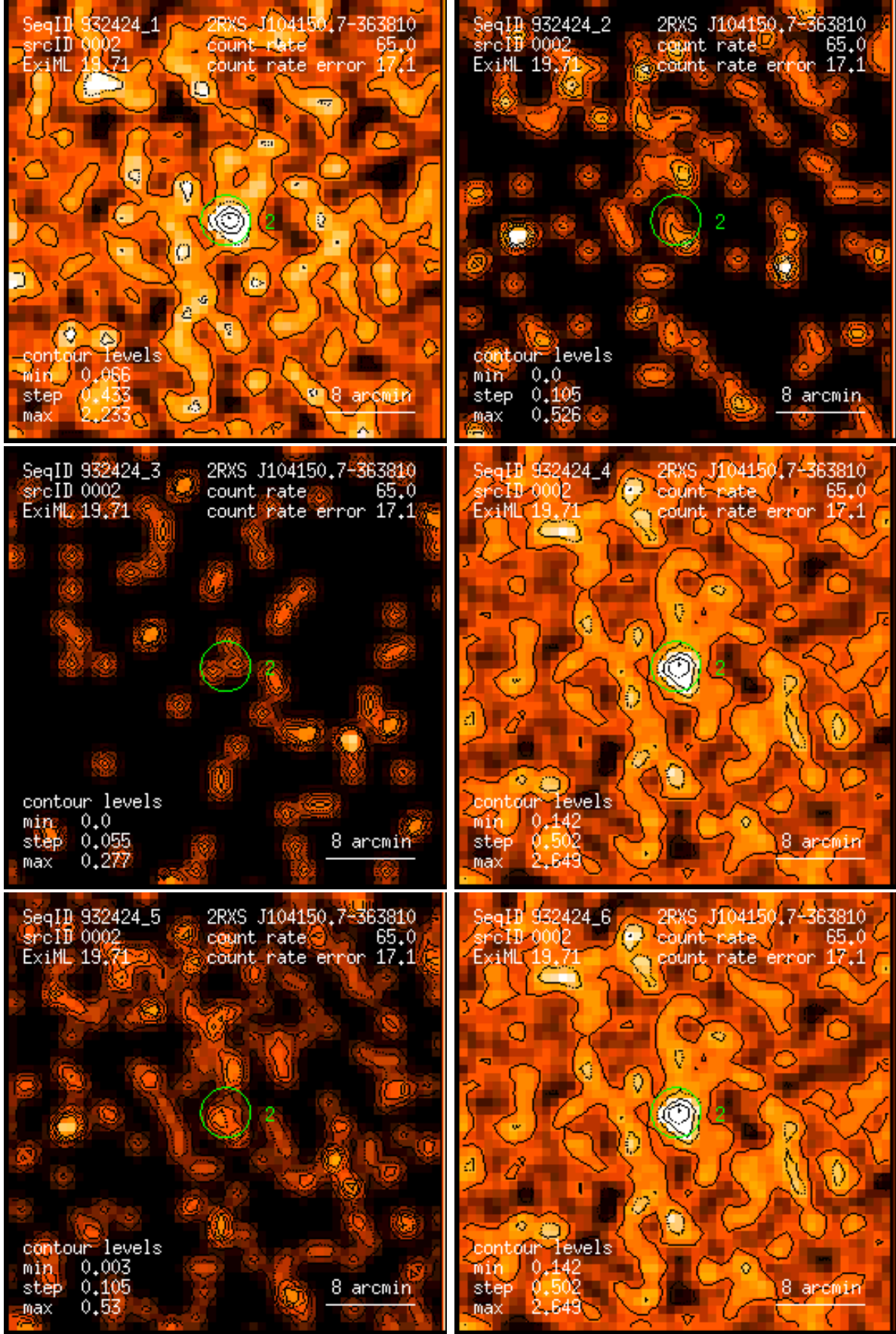
Figure 2: RASS 932424: detection 0002: band rate images, Gaussian filter: (1) PSPC channels 11 – 41, (2) 52 – 90, (3) 91 – 201, (4) 11 – 235, (5) 52 – 201, (6) 11 – 201. Broad band rates in counts/ks. Band rate contour levels in counts/ks/arcmin 2 .
