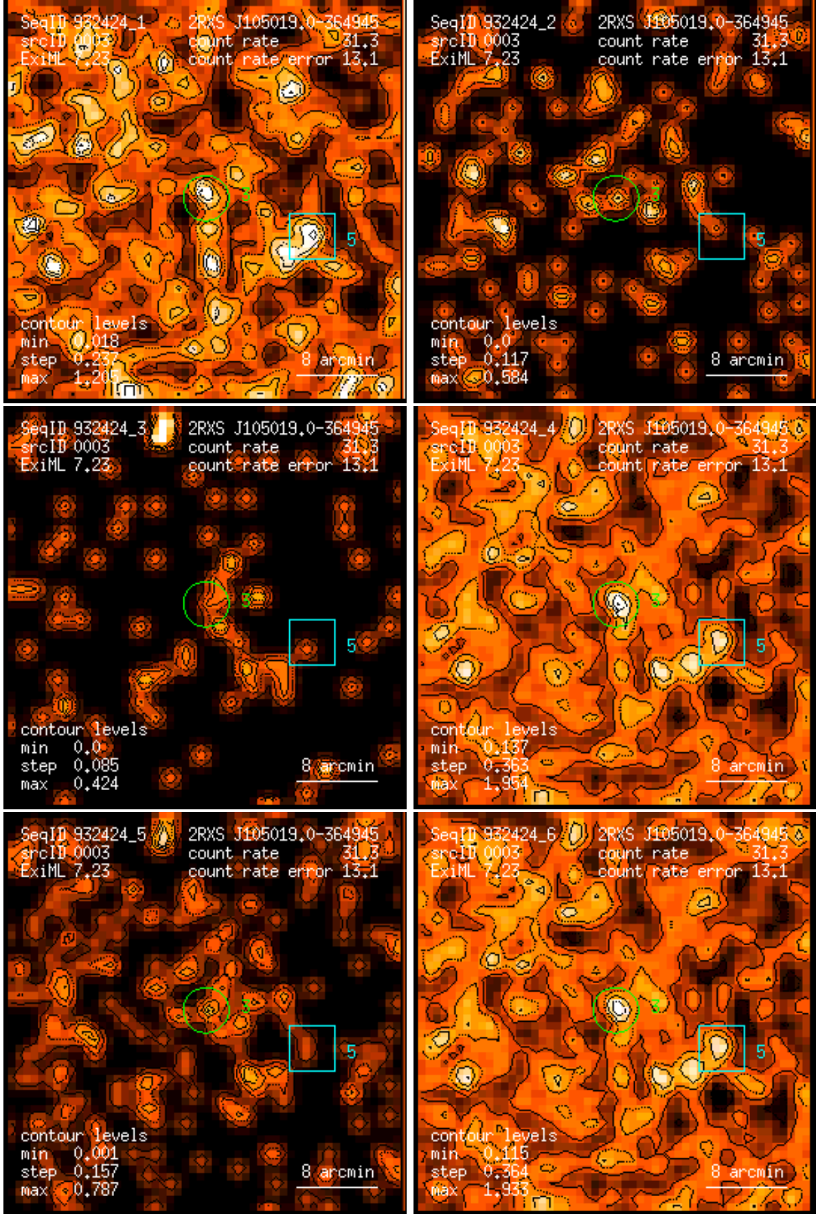
Figure 3: RASS 932424: detection 0003: band rate images, Gaussian filter: (1) PSPC channels 11 – 41, (2) 52 – 90, (3) 91 – 201, (4) 11 – 235, (5) 52 – 201, (6) 11 – 201. Broad band rates in counts/ks. Band rate contour levels in counts/ks/arcmin 2 .
