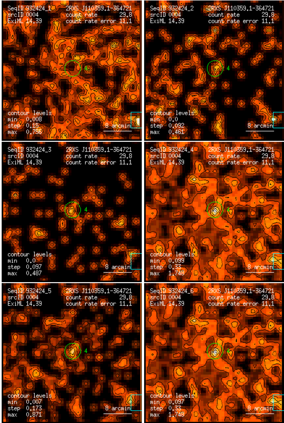
Figure 4: RASS 932424: detection 0004: band rate images, Gaussian filter: (1) PSPC channels 11 – 41, (2) 52 – 90, (3) 91 – 201, (4) 11 – 235, (5) 52 – 201, (6) 11 – 201. Broad band rates in counts/ks. Band rate contour levels in counts/ks/arcmin 2 .
