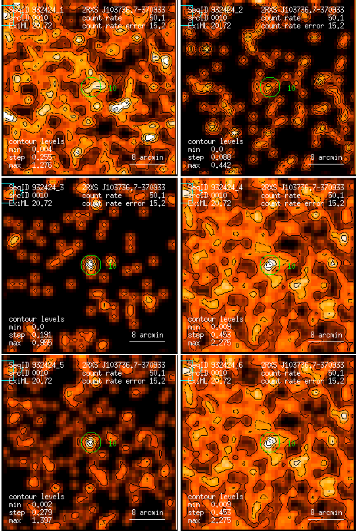
Figure 10: RASS 932424: detection 0010: band rate images, Gaussian filter: (1) PSPC channels 11 – 41, (2) 52 – 90, (3) 91 – 201, (4) 11 – 235, (5) 52 – 201, (6) 11 – 201. Broad band rates in counts/ks. Band rate contour levels in counts/ks/arcmin 2 .
