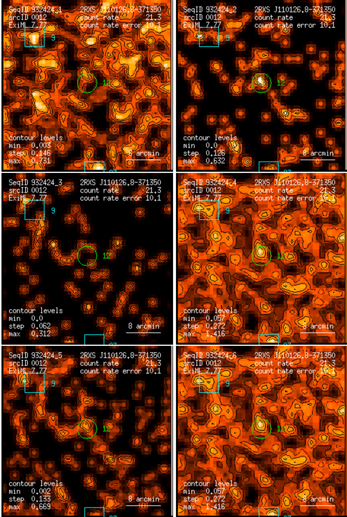
Figure 12: RASS 932424: detection 0012: band rate images, Gaussian filter: (1) PSPC channels 11 – 41, (2) 52 – 90, (3) 91 – 201, (4) 11 – 235, (5) 52 – 201, (6) 11 – 201. Broad band rates in counts/ks. Band rate contour levels in counts/ks/arcmin 2 .
