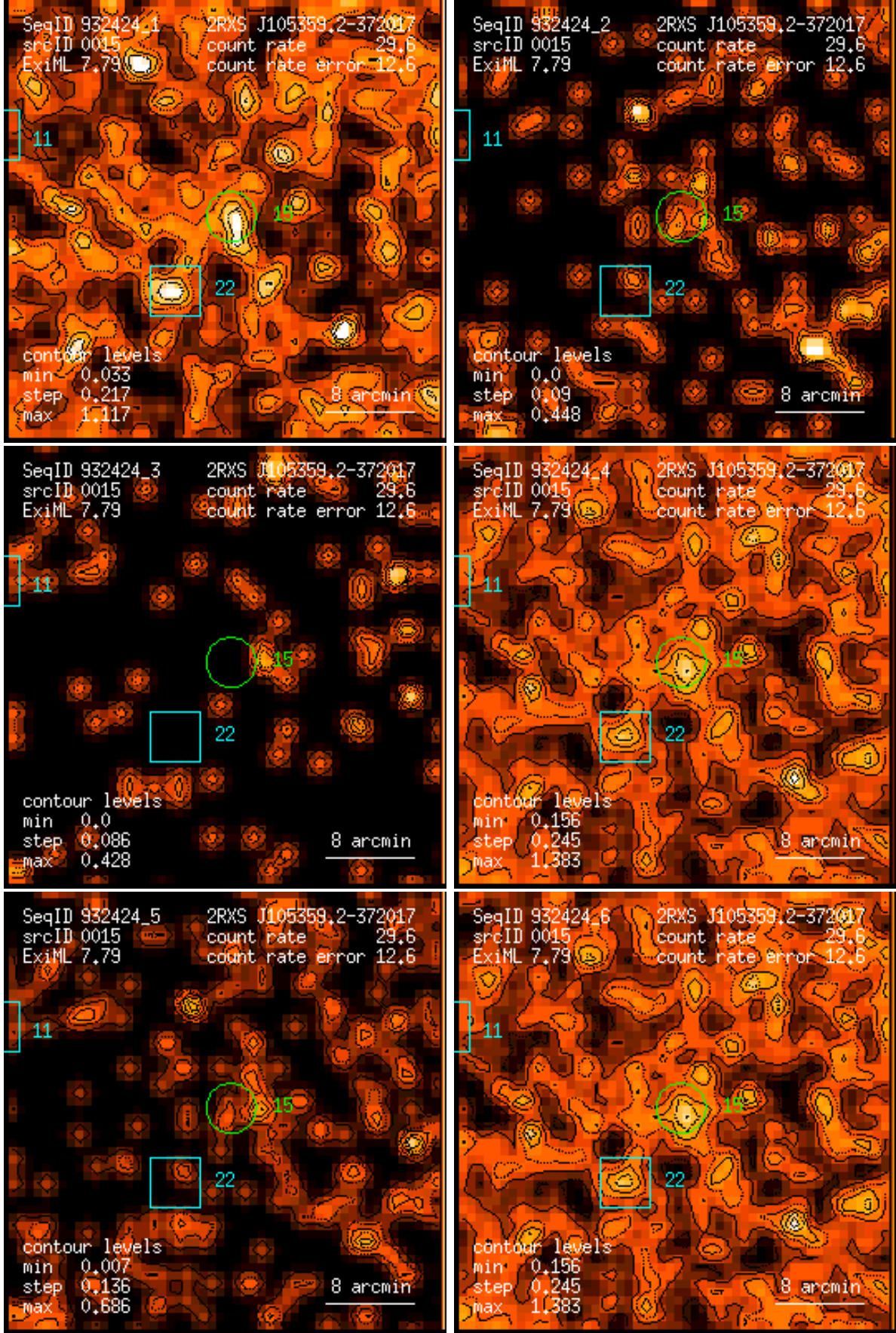
Figure 15: RASS 932424: detection 0015: band rate images, Gaussian filter: (1) PSPC channels 11 – 41, (2) 52 – 90, (3) 91 – 201, (4) 11 – 235, (5) 52 – 201, (6) 11 – 201. Broad band rates in counts/ks. Band rate contour levels in counts/ks/arcmin 2 .
