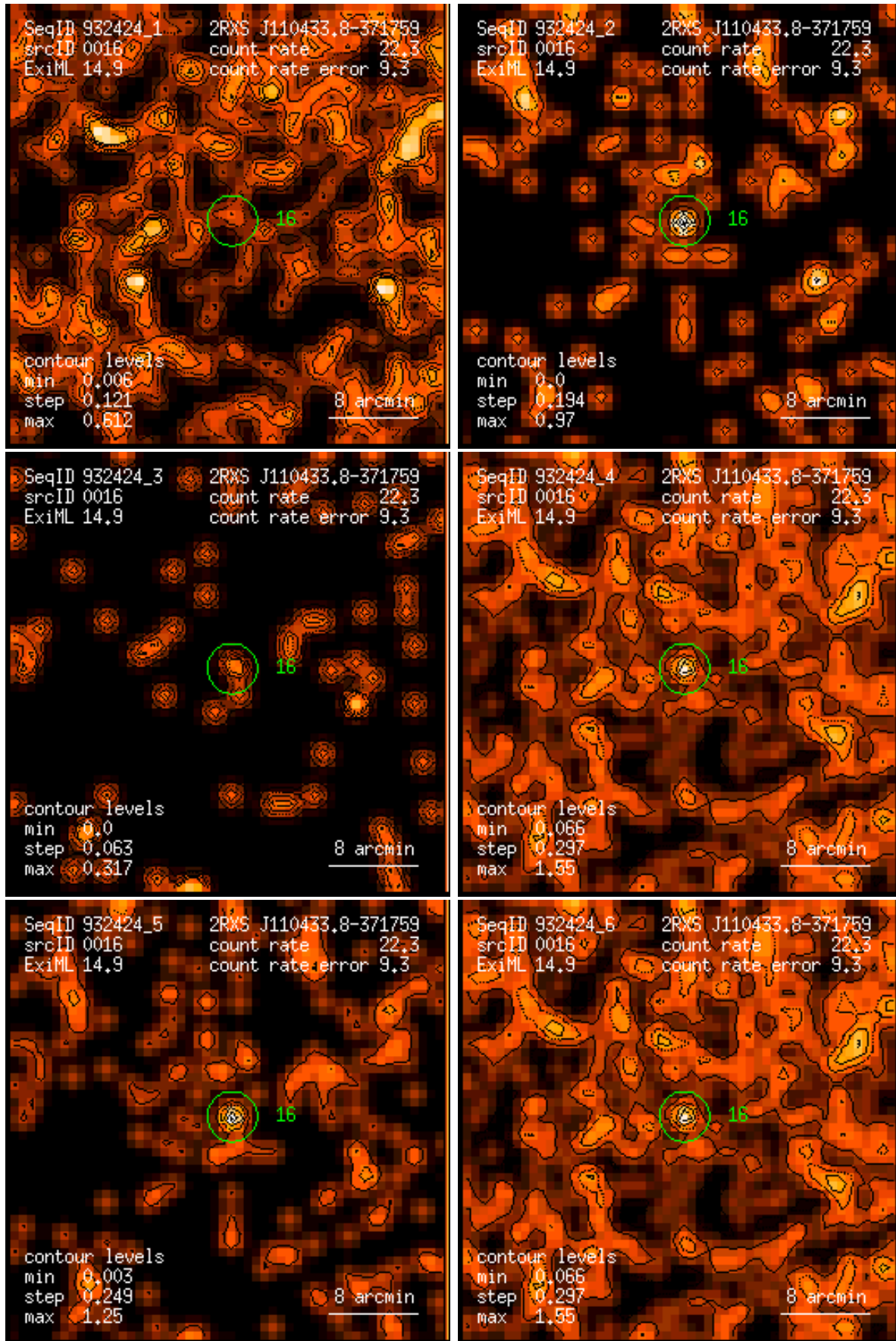
Figure 16: RASS 932424: detection 0016: band rate images, Gaussian filter: (1) PSPC channels 11 – 41, (2) 52 – 90, (3) 91 – 201, (4) 11 – 235, (5) 52 – 201, (6) 11 – 201. Broad band rates in counts/ks. Band rate contour levels in counts/ks/arcmin 2 .
