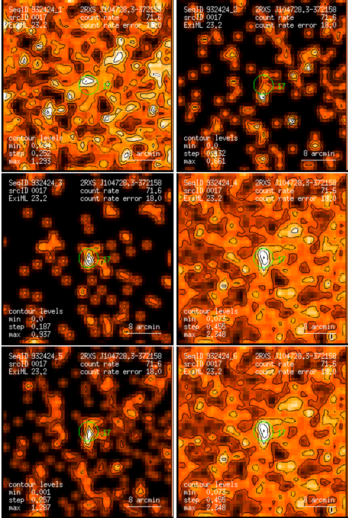
Figure 17: RASS 932424: detection 0017: band rate images, Gaussian filter: (1) PSPC channels 11 – 41, (2) 52 – 90, (3) 91 – 201, (4) 11 – 235, (5) 52 – 201, (6) 11 – 201. Broad band rates in counts/ks. Band rate contour levels in counts/ks/arcmin 2 .
