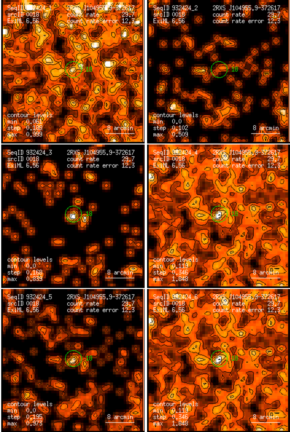
Figure 18: RASS 932424: detection 0018: band rate images, Gaussian filter: (1) PSPC channels 11 – 41, (2) 52 – 90, (3) 91 – 201, (4) 11 – 235, (5) 52 – 201, (6) 11 – 201. Broad band rates in counts/ks. Band rate contour levels in counts/ks/arcmin 2 .
