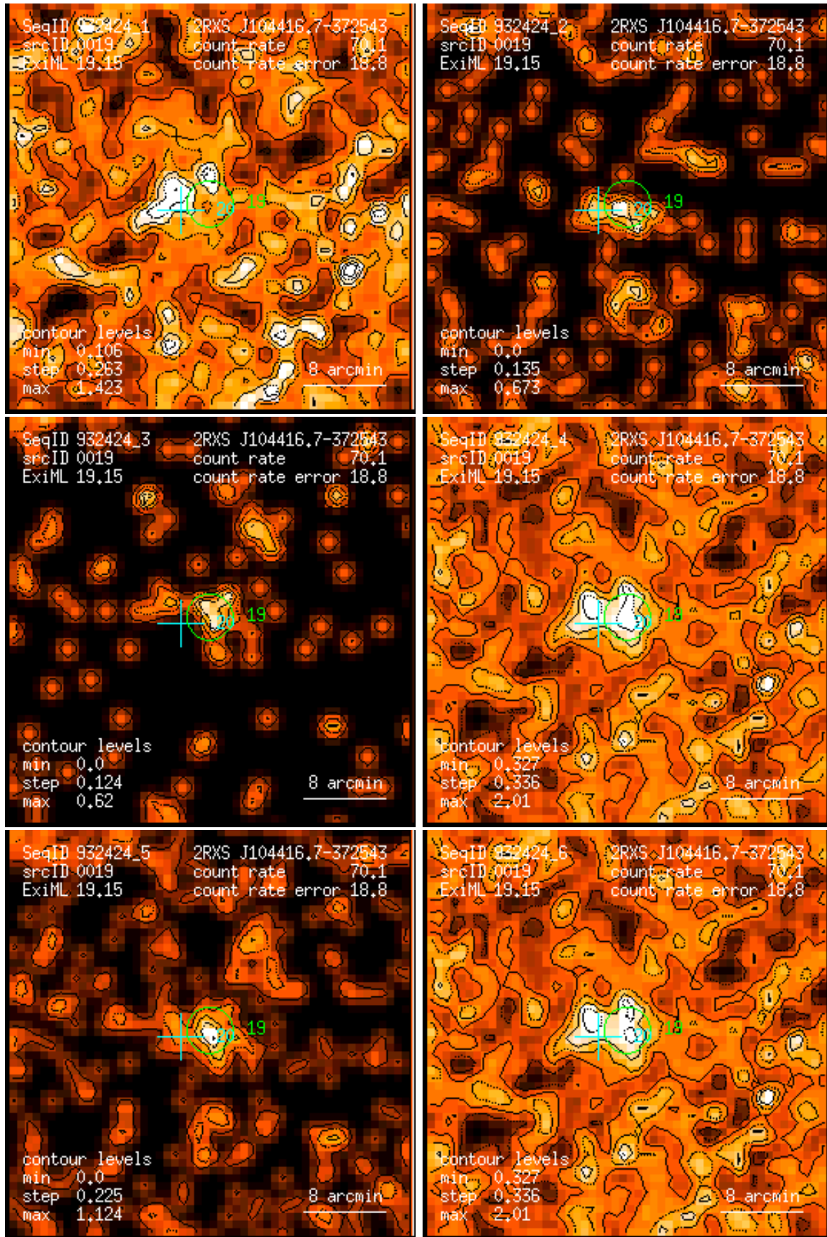
Figure 19: RASS 932424: detection 0019: band rate images, Gaussian filter: (1) PSPC channels 11 – 41, (2) 52 – 90, (3) 91 – 201, (4) 11 – 235, (5) 52 – 201, (6) 11 – 201. Broad band rates in counts/ks. Band rate contour levels in counts/ks/arcmin 2 .
