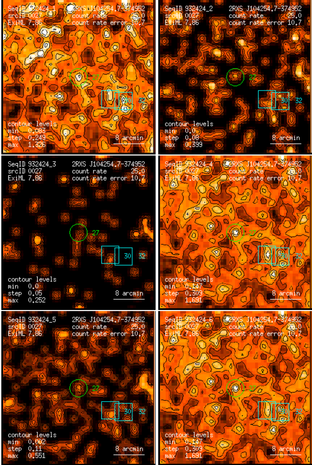
Figure 27: RASS 932424: detection 0027: band rate images, Gaussian filter: (1) PSPC channels 11 – 41, (2) 52 – 90, (3) 91 – 201, (4) 11 – 235, (5) 52 – 201, (6) 11 – 201. Broad band rates in counts/ks. Band rate contour levels in counts/ks/arcmin 2 .
