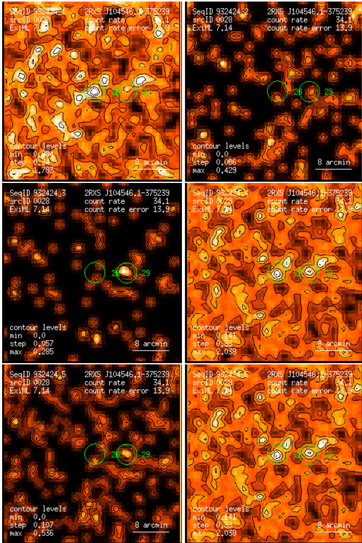
Figure 28: RASS 932424: detection 0028: band rate images, Gaussian filter: (1) PSPC channels 11 – 41, (2) 52 – 90, (3) 91 – 201, (4) 11 – 235, (5) 52 – 201, (6) 11 – 201. Broad band rates in counts/ks. Band rate contour levels in counts/ks/arcmin 2 .
