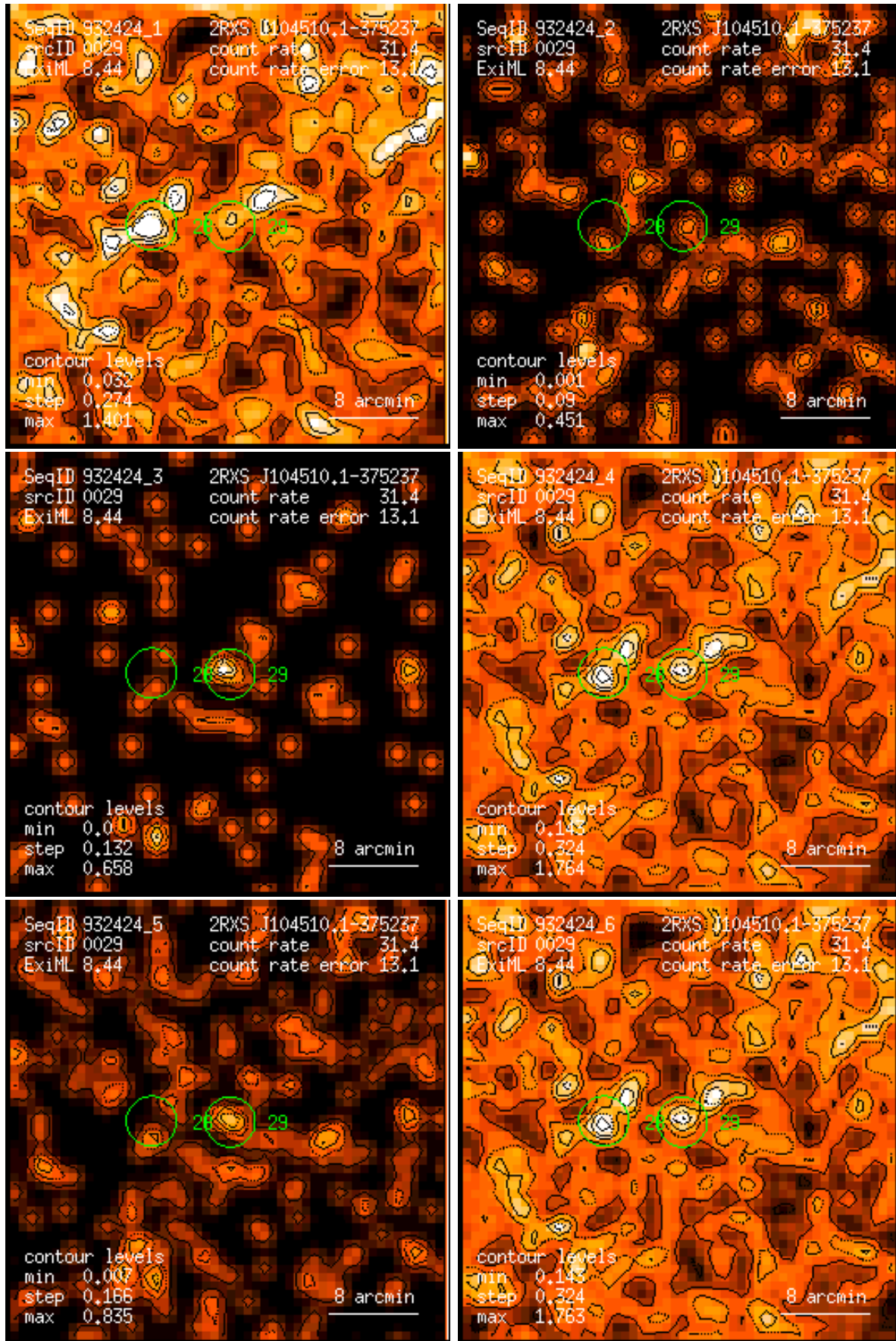
Figure 29: RASS 932424: detection 0029: band rate images, Gaussian filter: (1) PSPC channels 11 – 41, (2) 52 – 90, (3) 91 – 201, (4) 11 – 235, (5) 52 – 201, (6) 11 – 201. Broad band rates in counts/ks. Band rate contour levels in counts/ks/arcmin 2 .
