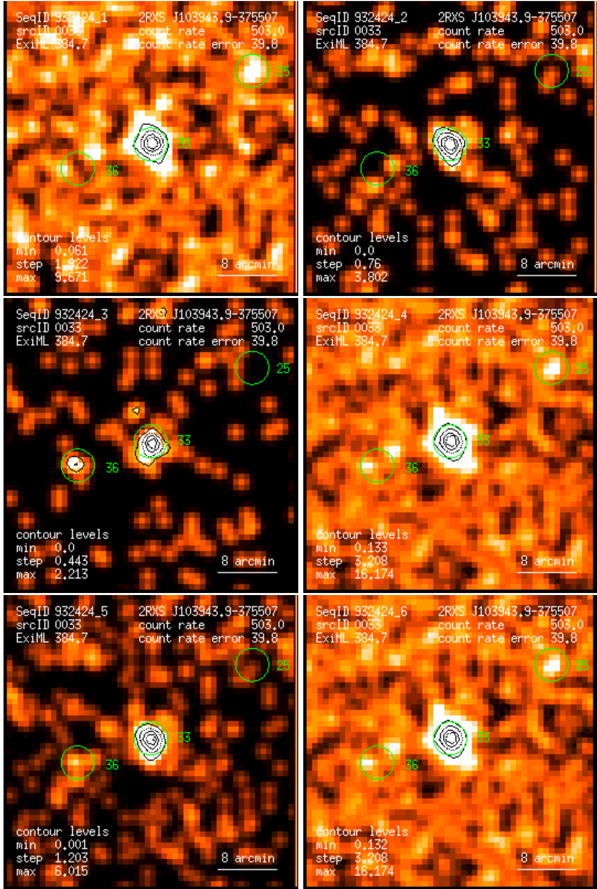
Figure 33: RASS 932424: detection 0033: band rate images, Gaussian filter: (1) PSPC channels 11 – 41, (2) 52 – 90, (3) 91 – 201, (4) 11 – 235, (5) 52 – 201, (6) 11 – 201. Broad band rates in counts/ks. Band rate contour levels in counts/ks/arcmin 2 .
