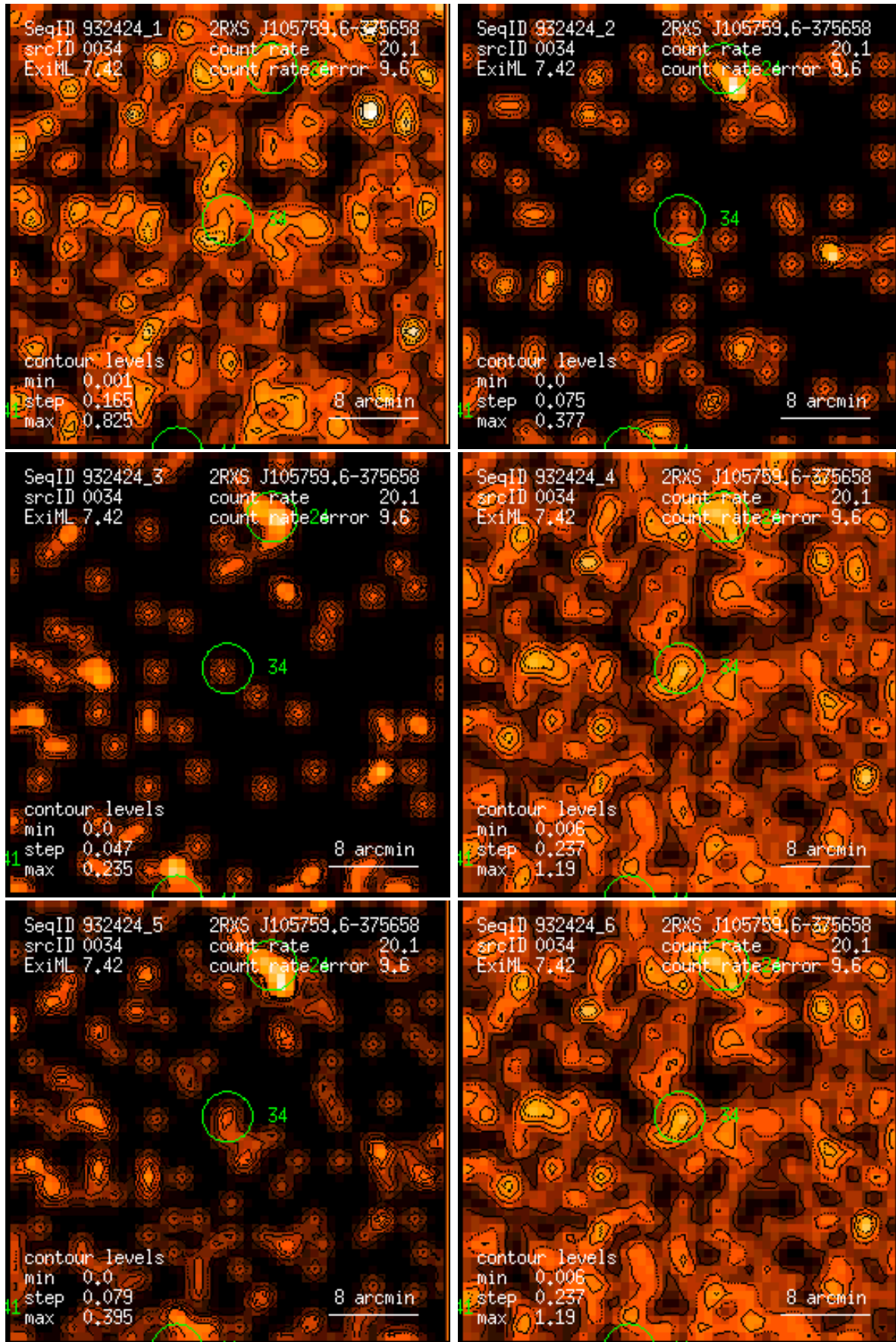
Figure 34: RASS 932424: detection 0034: band rate images, Gaussian filter: (1) PSPC channels 11 – 41, (2) 52 – 90, (3) 91 – 201, (4) 11 – 235, (5) 52 – 201, (6) 11 – 201. Broad band rates in counts/ks. Band rate contour levels in counts/ks/arcmin 2 .
