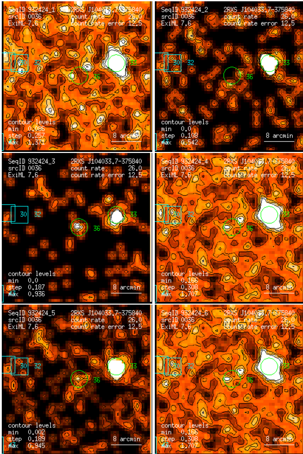
Figure 36: RASS 932424: detection 0036: band rate images, Gaussian filter: (1) PSPC channels 11 – 41, (2) 52 – 90, (3) 91 – 201, (4) 11 – 235, (5) 52 – 201, (6) 11 – 201. Broad band rates in counts/ks. Band rate contour levels in counts/ks/arcmin 2 .
