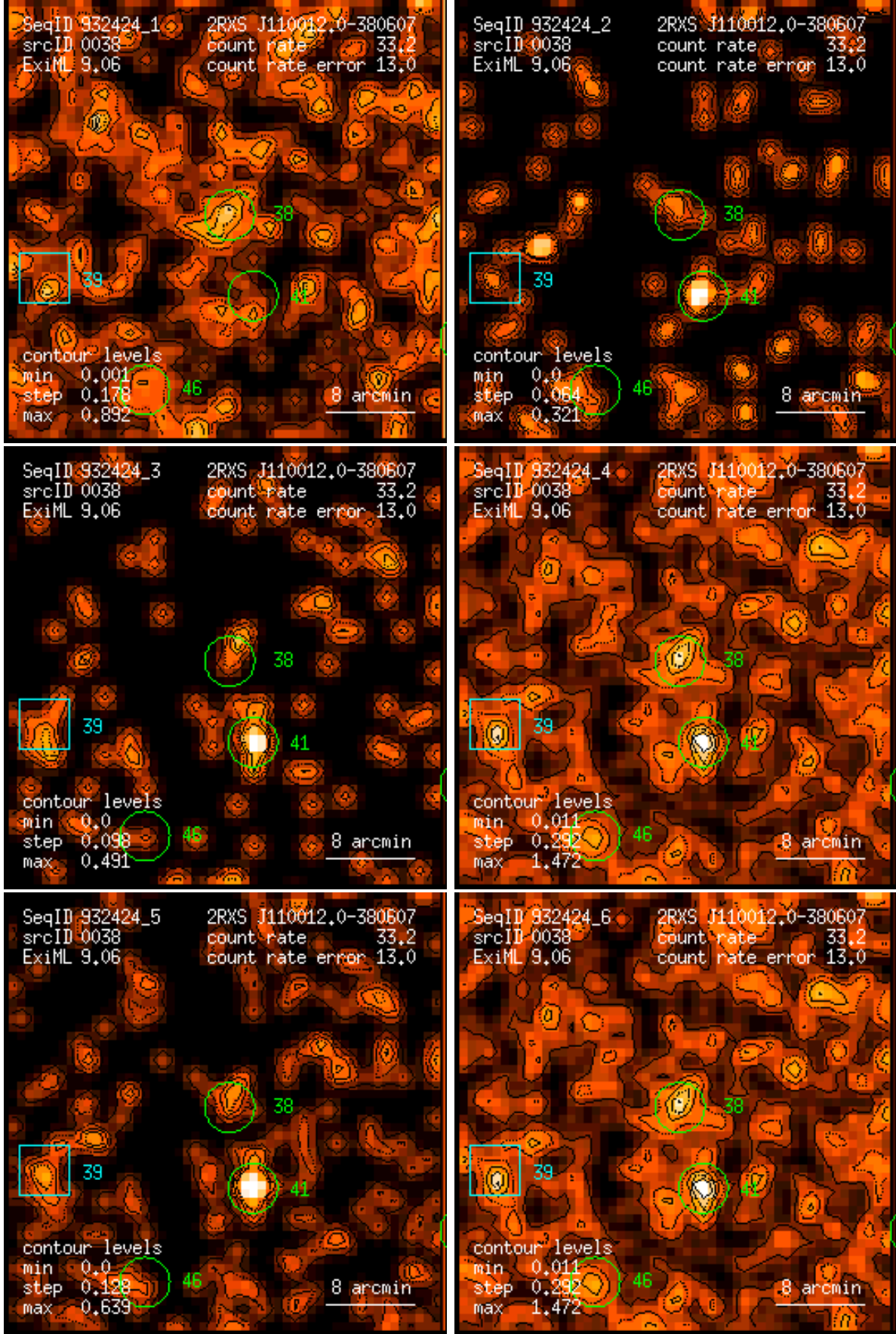
Figure 38: RASS 932424: detection 0038: band rate images, Gaussian filter: (1) PSPC channels 11 – 41, (2) 52 – 90, (3) 91 – 201, (4) 11 – 235, (5) 52 – 201, (6) 11 – 201. Broad band rates in counts/ks. Band rate contour levels in counts/ks/arcmin 2 .
