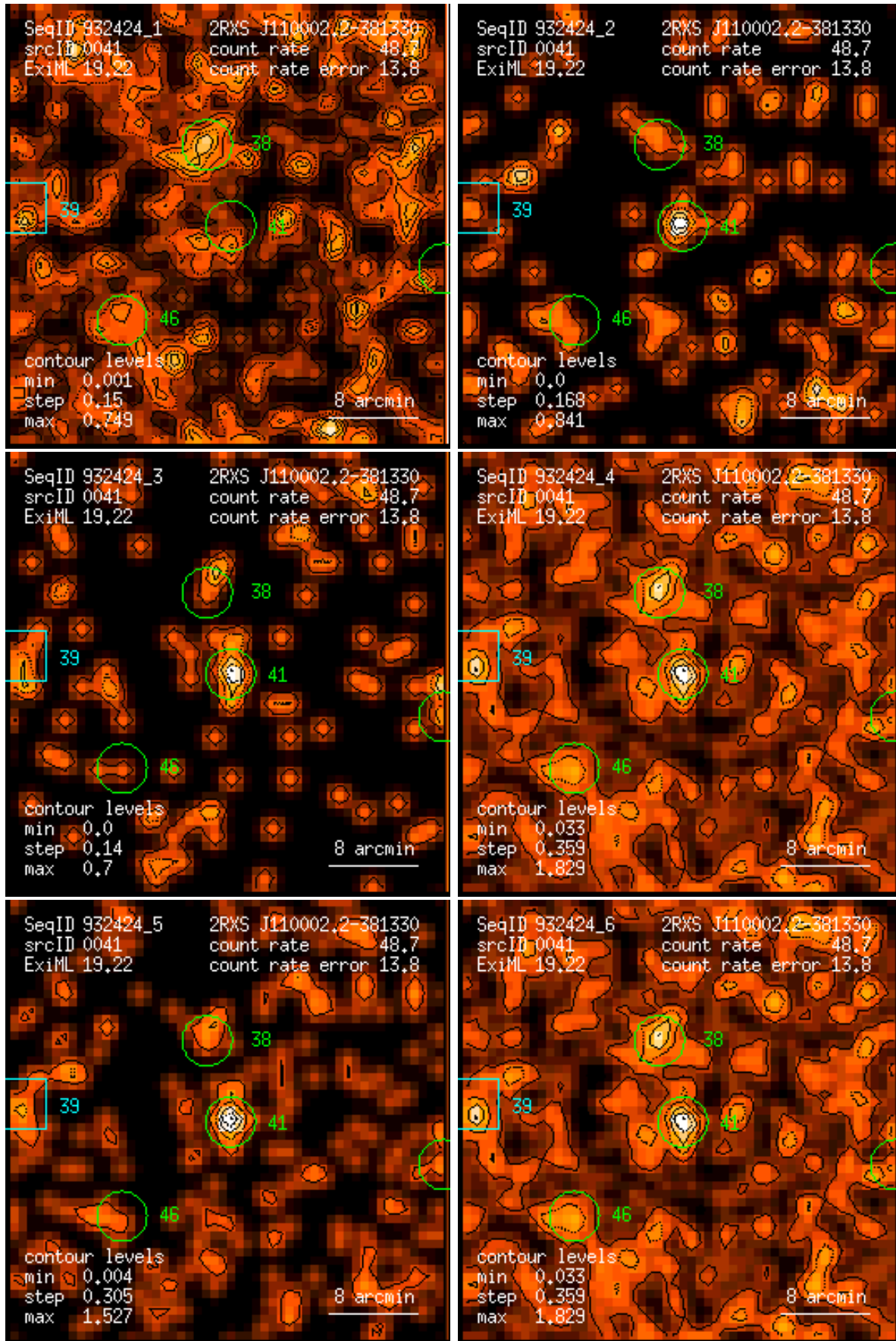
Figure 41: RASS 932424: detection 0041: band rate images, Gaussian filter: (1) PSPC channels 11 – 41, (2) 52 – 90, (3) 91 – 201, (4) 11 – 235, (5) 52 – 201, (6) 11 – 201. Broad band rates in counts/ks. Band rate contour levels in counts/ks/arcmin 2 .
