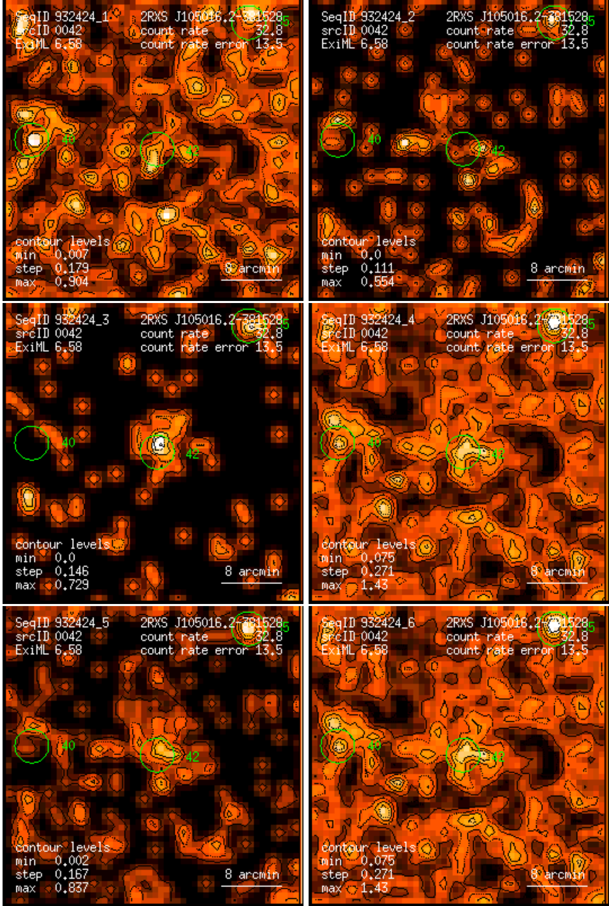
Figure 42: RASS 932424: detection 0042: band rate images, Gaussian filter: (1) PSPC channels 11 – 41, (2) 52 – 90, (3) 91 – 201, (4) 11 – 235, (5) 52 – 201, (6) 11 – 201. Broad band rates in counts/ks. Band rate contour levels in counts/ks/arcmin 2 .
