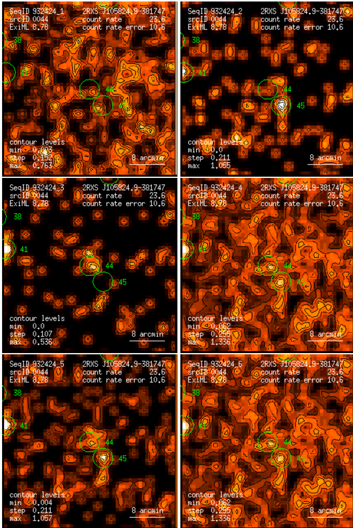
Figure 44: RASS 932424: detection 0044: band rate images, Gaussian filter: (1) PSPC channels 11 – 41, (2) 52 – 90, (3) 91 – 201, (4) 11 – 235, (5) 52 – 201, (6) 11 – 201. Broad band rates in counts/ks. Band rate contour levels in counts/ks/arcmin 2 .
