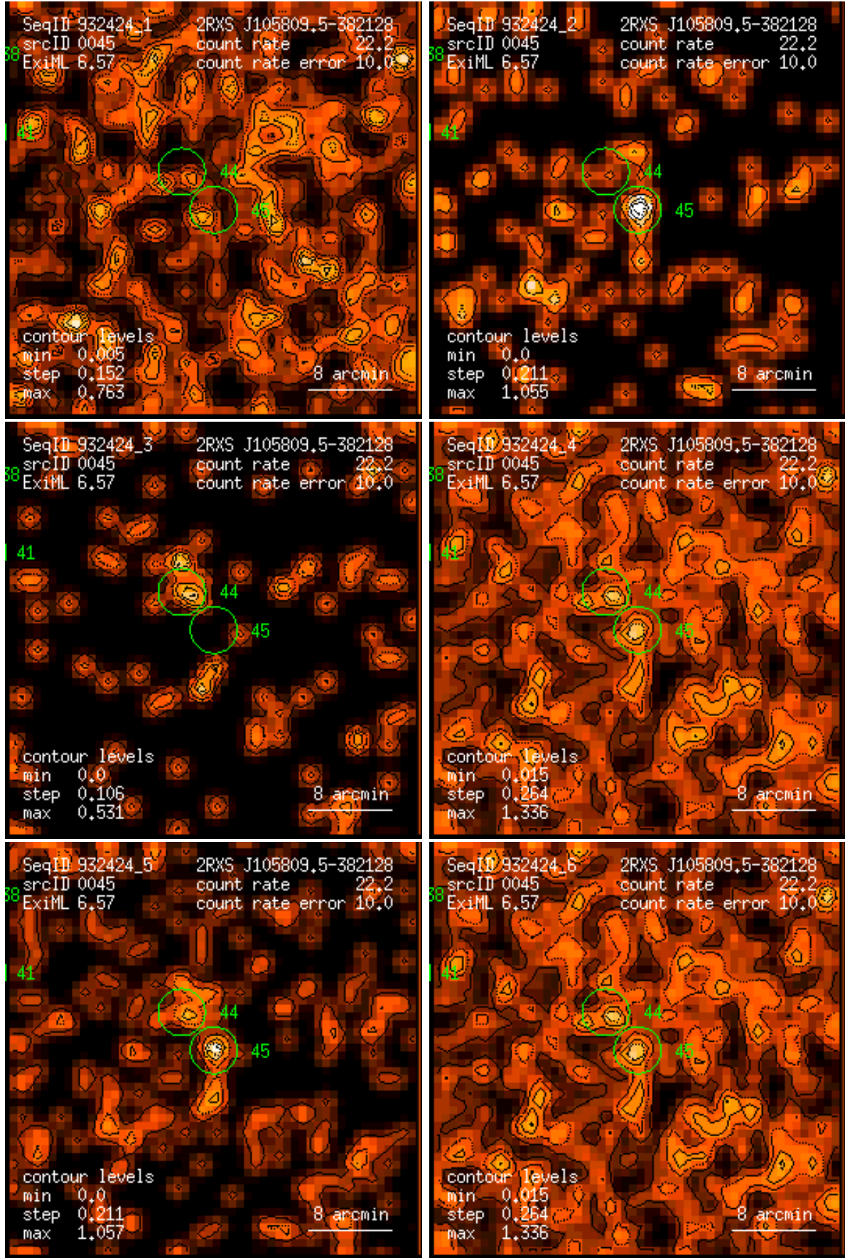
Figure 45: RASS 932424: detection 0045: band rate images, Gaussian filter: (1) PSPC channels 11 – 41, (2) 52 – 90, (3) 91 – 201, (4) 11 – 235, (5) 52 – 201, (6) 11 – 201. Broad band rates in counts/ks. Band rate contour levels in counts/ks/arcmin 2 .
