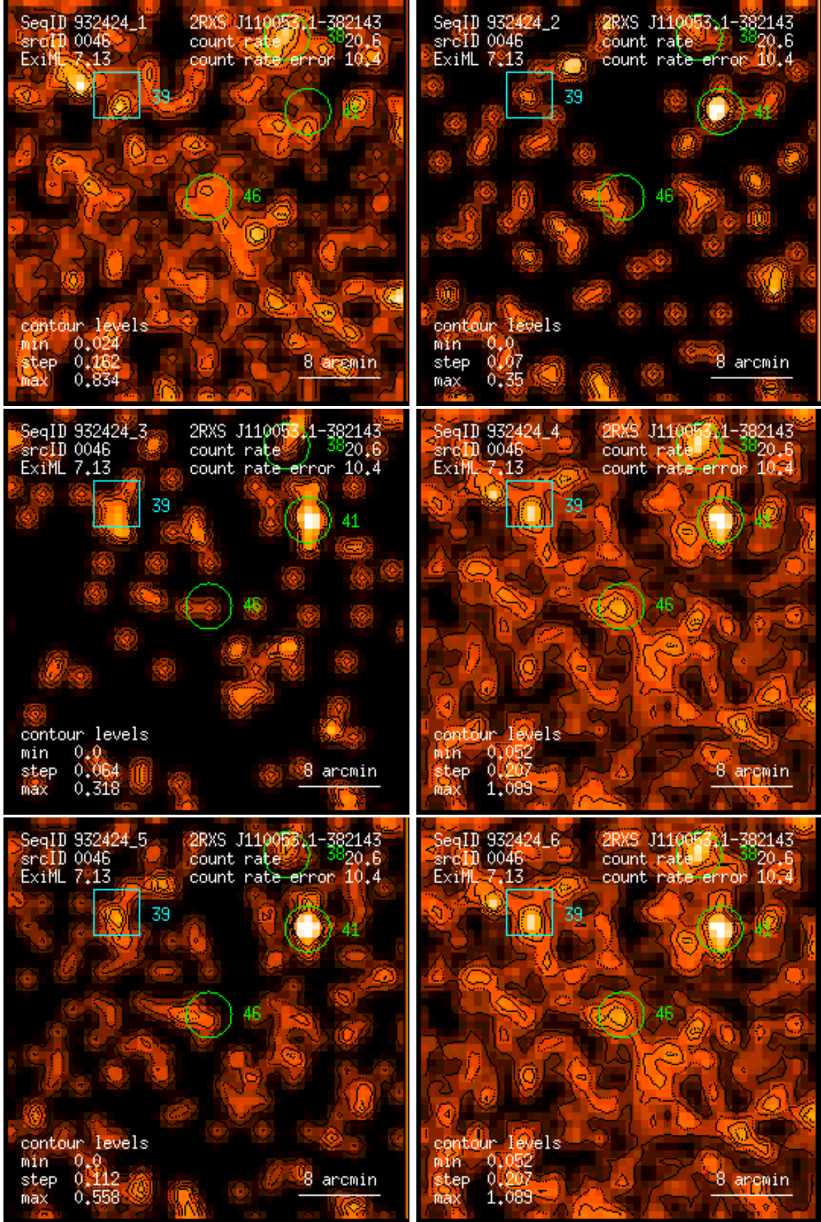
Figure 46: RASS 932424: detection 0046: band rate images, Gaussian filter: (1) PSPC channels 11 – 41, (2) 52 – 90, (3) 91 – 201, (4) 11 – 235, (5) 52 – 201, (6) 11 – 201. Broad band rates in counts/ks. Band rate contour levels in counts/ks/arcmin 2 .
