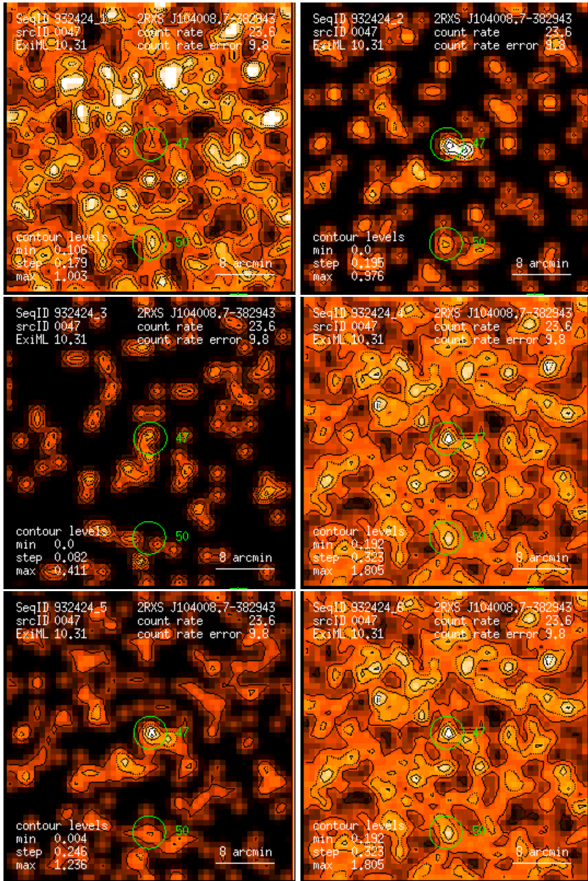
Figure 47: RASS 932424: detection 0047: band rate images, Gaussian filter: (1) PSPC channels 11 – 41, (2) 52 – 90, (3) 91 – 201, (4) 11 – 235, (5) 52 – 201, (6) 11 – 201. Broad band rates in counts/ks. Band rate contour levels in counts/ks/arcmin 2 .
