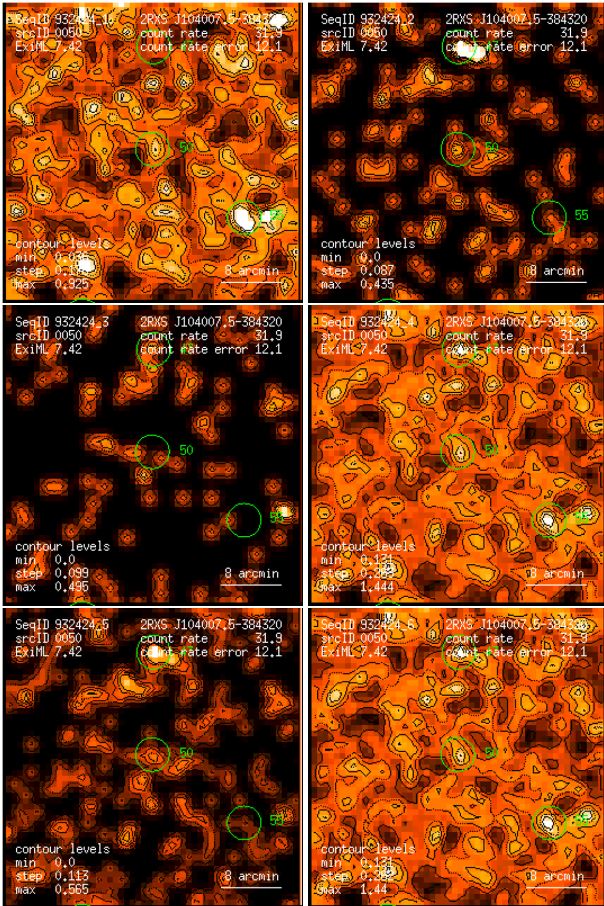
Figure 50: RASS 932424: detection 0050: band rate images, Gaussian filter: (1) PSPC channels 11 – 41, (2) 52 – 90, (3) 91 – 201, (4) 11 – 235, (5) 52 – 201, (6) 11 – 201. Broad band rates in counts/ks. Band rate contour levels in counts/ks/arcmin 2 .
