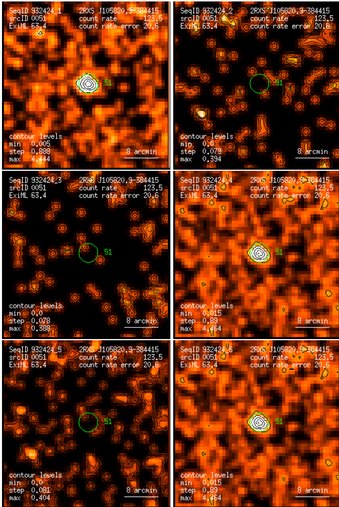
Figure 51: RASS 932424: detection 0051: band rate images, Gaussian filter: (1) PSPC channels 11 – 41, (2) 52 – 90, (3) 91 – 201, (4) 11 – 235, (5) 52 – 201, (6) 11 – 201. Broad band rates in counts/ks. Band rate contour levels in counts/ks/arcmin 2 .
