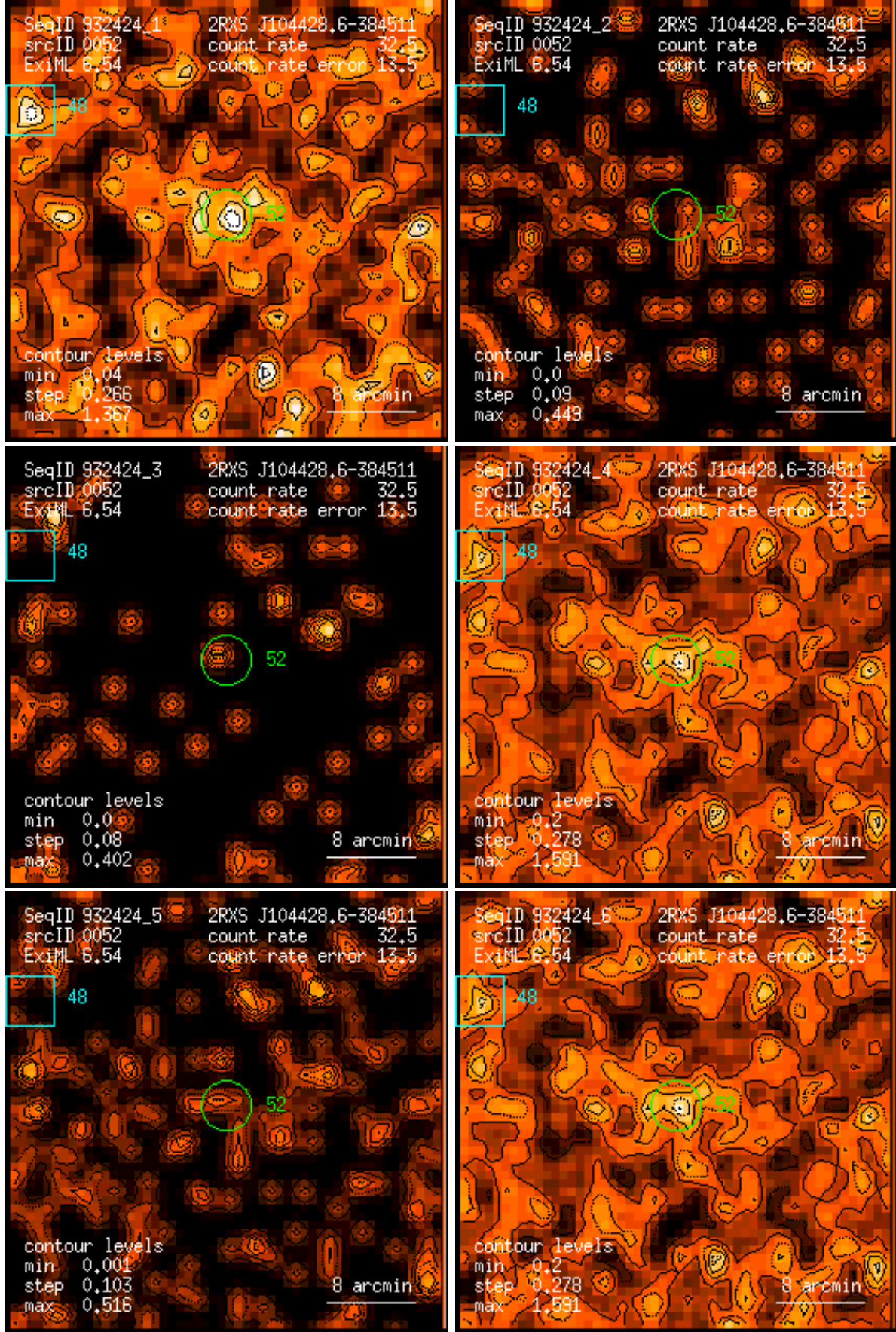
Figure 52: RASS 932424: detection 0052: band rate images, Gaussian filter: (1) PSPC channels 11 – 41, (2) 52 – 90, (3) 91 – 201, (4) 11 – 235, (5) 52 – 201, (6) 11 – 201. Broad band rates in counts/ks. Band rate contour levels in counts/ks/arcmin 2 .
